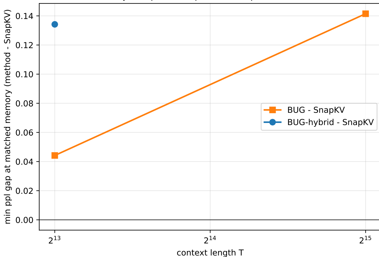
Does the hybrid pass SnapKV where pure BUG could not?
