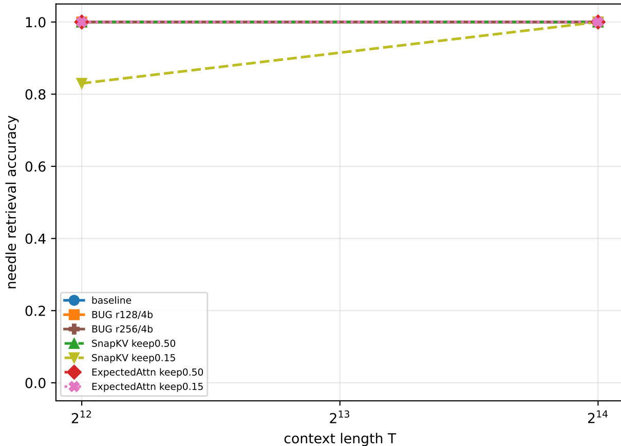
Experiment B: retrieval vs context (matched memory)
