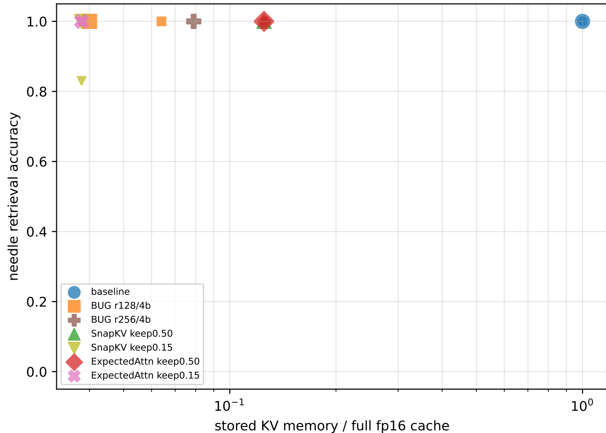
accuracy vs memory (marker size ~ ctx)
