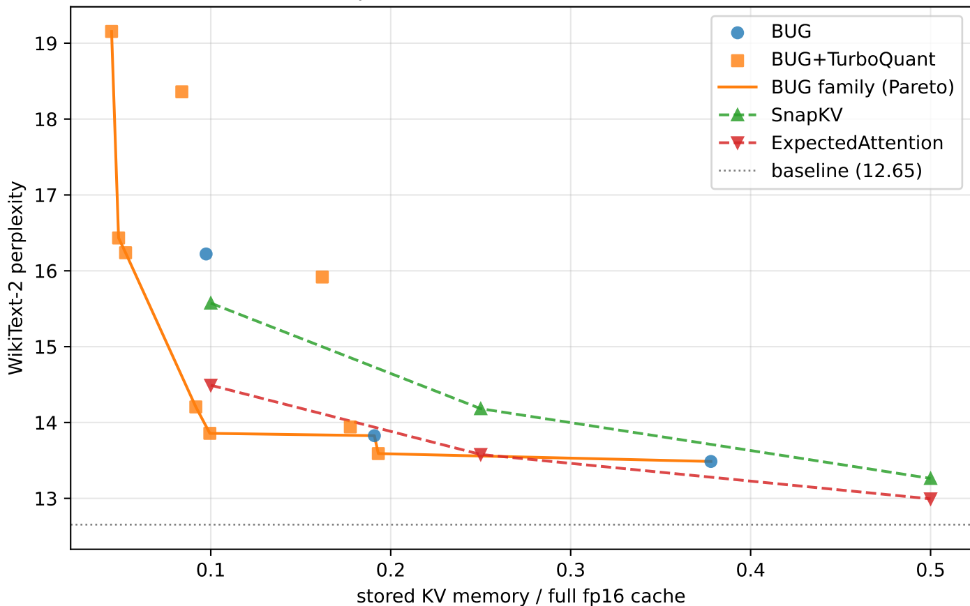
KV-cache compression — Llama-3.2-1B-Instruct, ctx 1024
