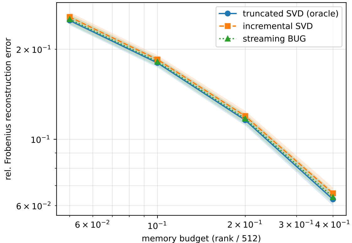
Layer-8 K, pre-RoPE
