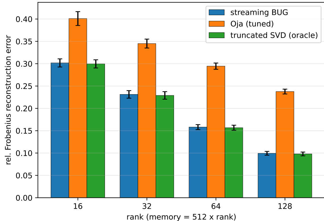
Layer-8 K, pre-RoPE
