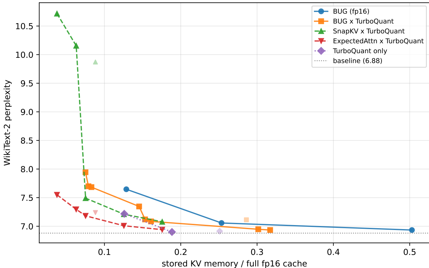
Fair: every mechanism x TurboQuant — Meta-Llama-3.1-8B-Instruct, ctx 1024
