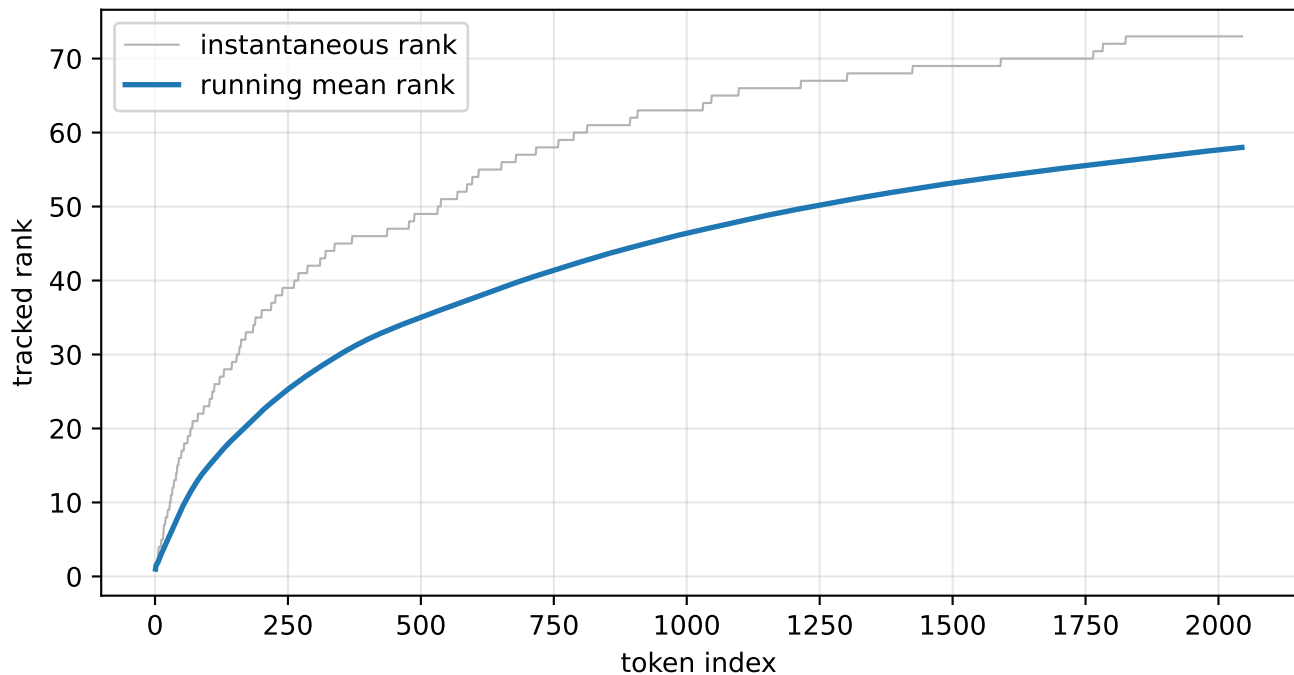
Streaming BUG rank vs. token (Layer 8, \theta=20 )
