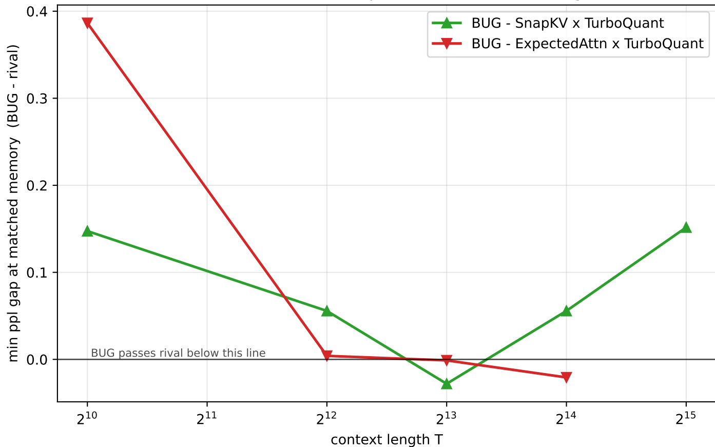
Axis C: does BUG's frontier pass eviction as context grows?
