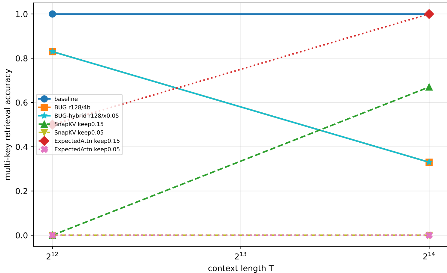
RULER-lite: retrieve 1 of N keys under aggressive compression
