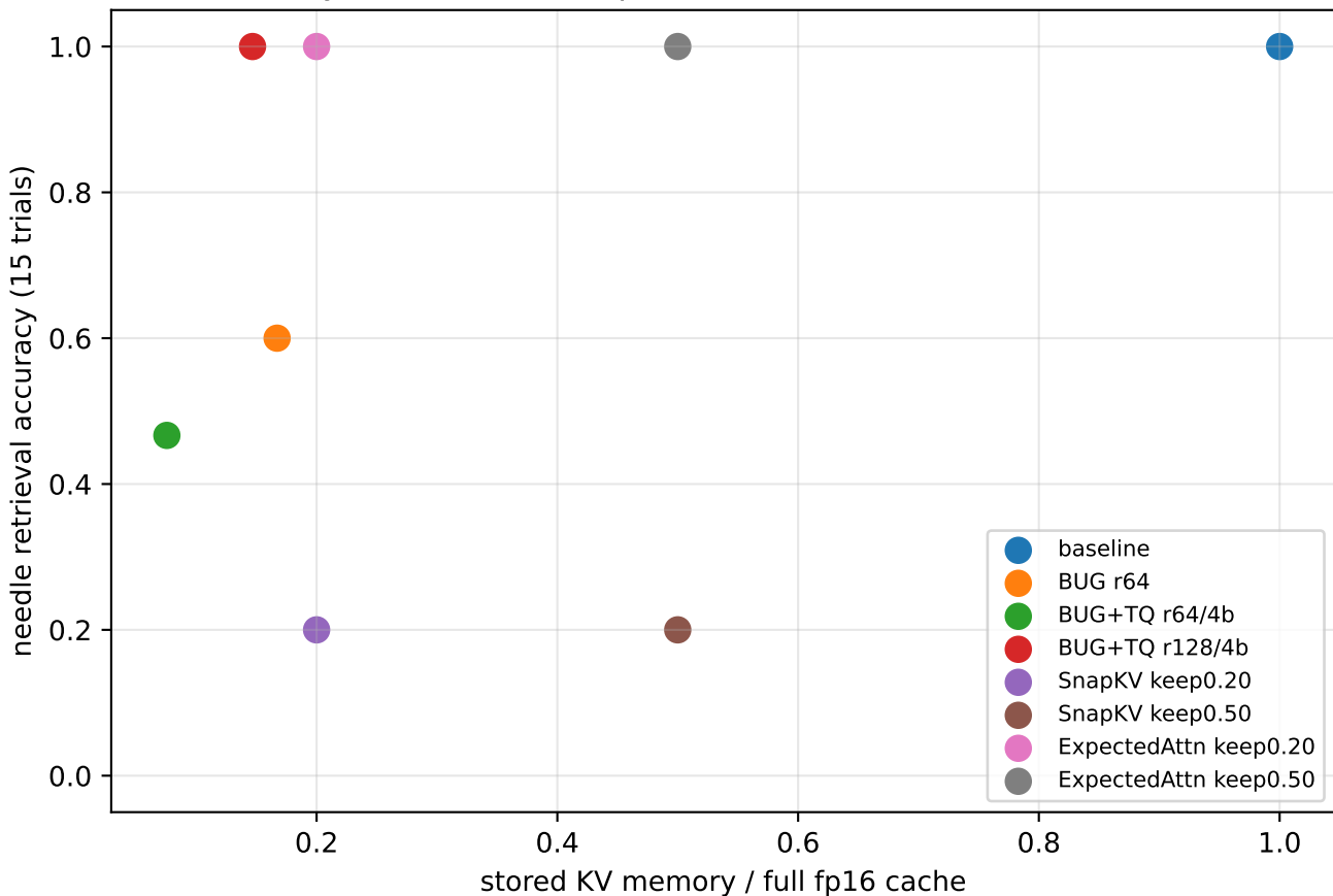
Needle-in-haystack under compression — Llama-3.2-1B-Instruct, ctx 1600
