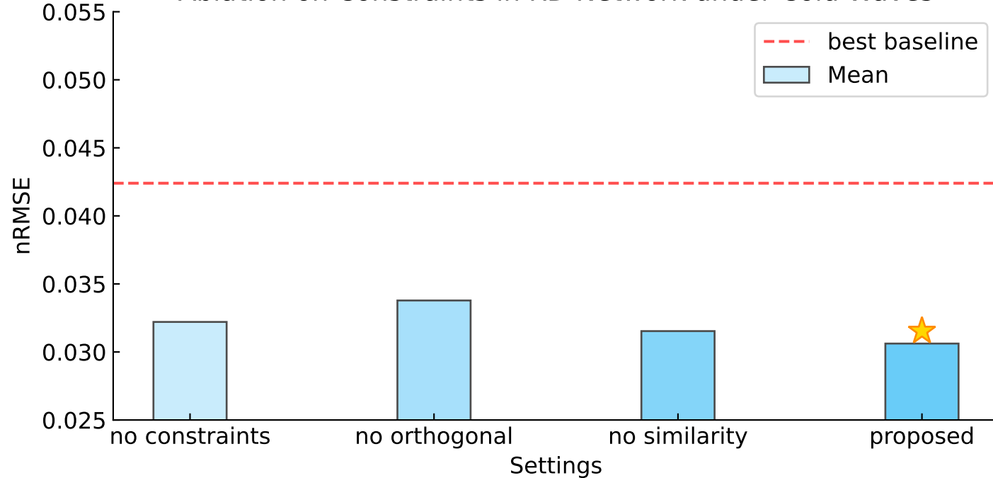
Ablation on Constraints in RD Network under Cold Waves
