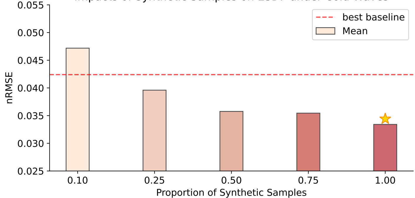
Impacts of Synthetic Samples on ESDF under Cold Waves
