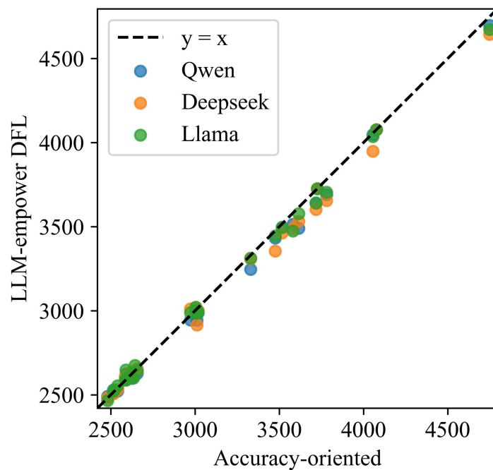
Tree+LP
