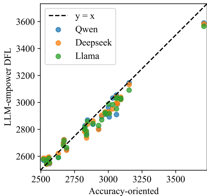
NN+LP
