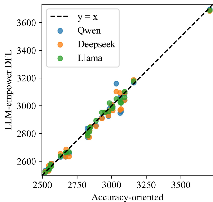
NN+MILP
