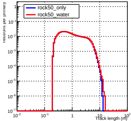
Backscattered neutrons, all energies
