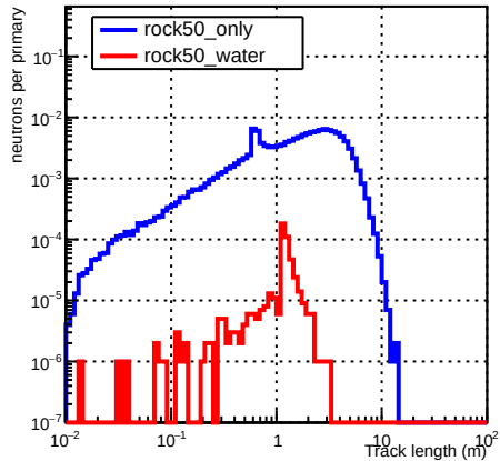
Transmitted neutrons
