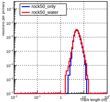
Backscattered thermal neutrons ( < 0.5 eV)
