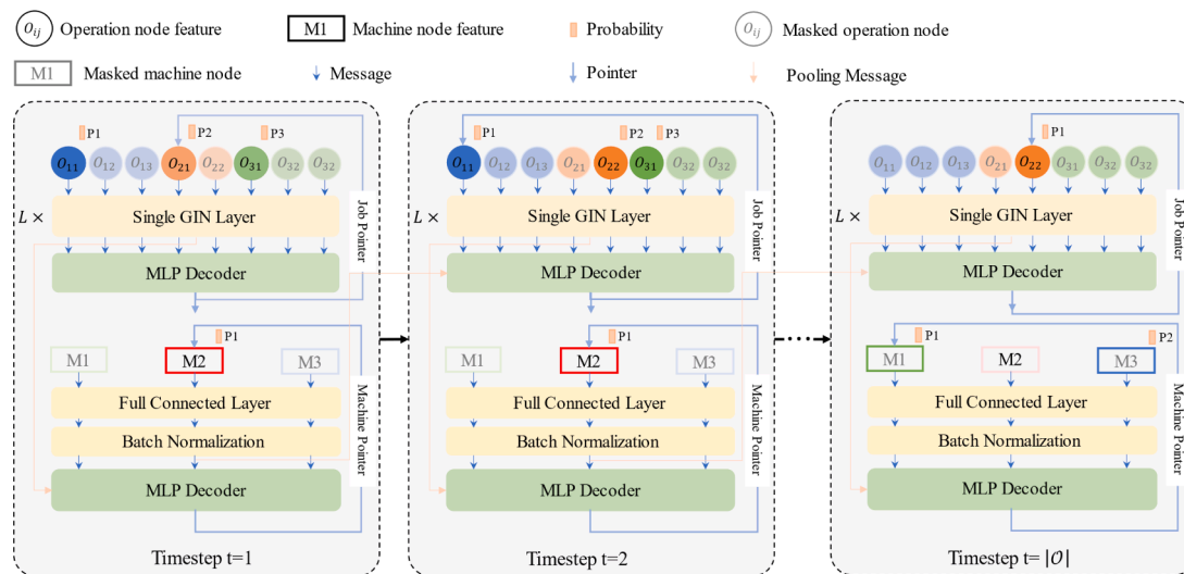
Fig. 3. The MPGN architecture for the FJSP.
