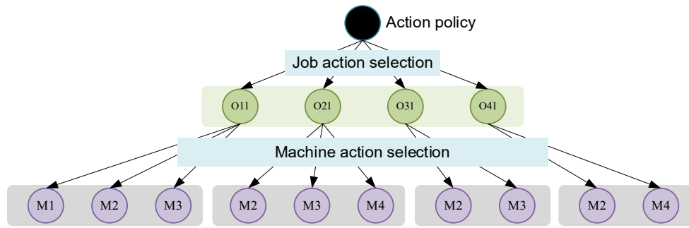
Fig. 1. Illustration of the multi-action space for FJSP.
