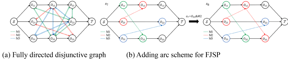
Fig. 4. Fully directed disjunctive graph and adding arc scheme for FJSP.
