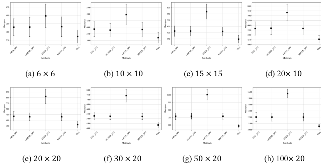
Fig. 8. Means plot and 95% confidence level Tukey's HSD intervals for solution values of 128 instances of different methods and scales.
