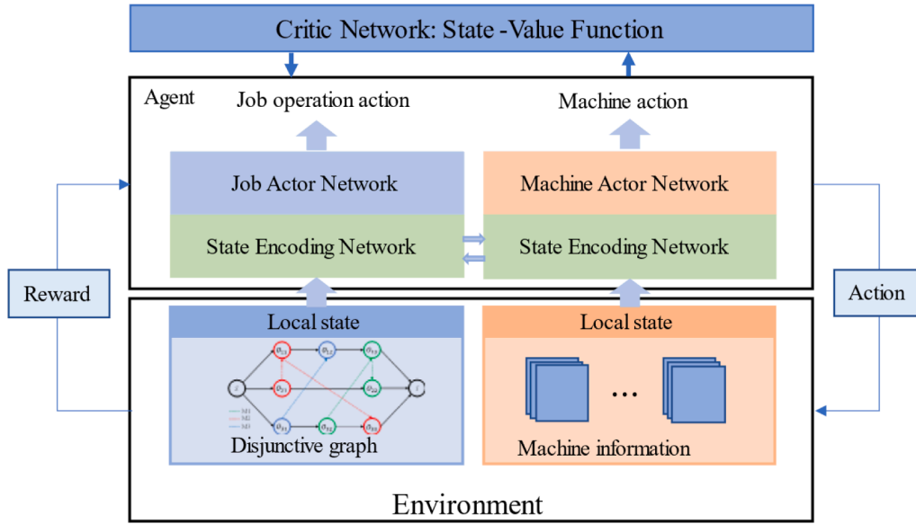
Fig. 5. Multiple actor-critic architecture for a multi-action space scheduling problem.
