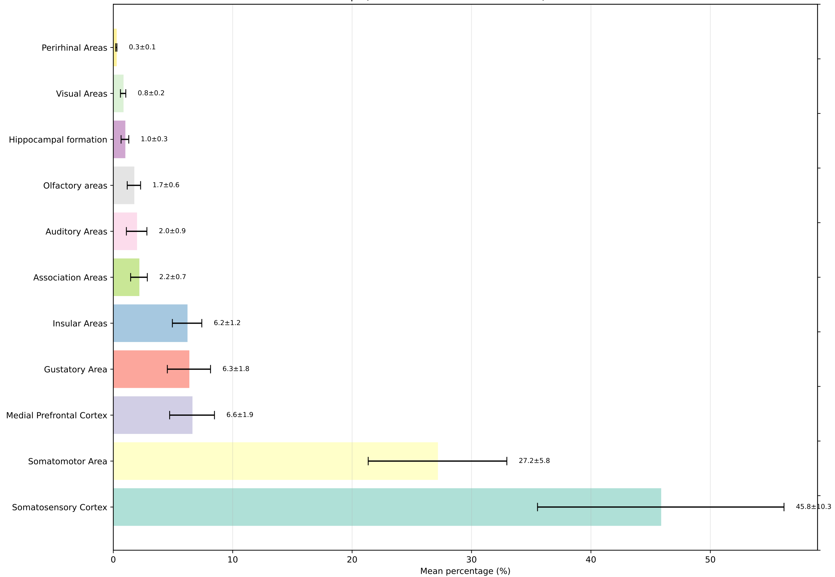
Custom Cortical Groups (Normalized to 100% within Cortex) with Individual Brain Values
