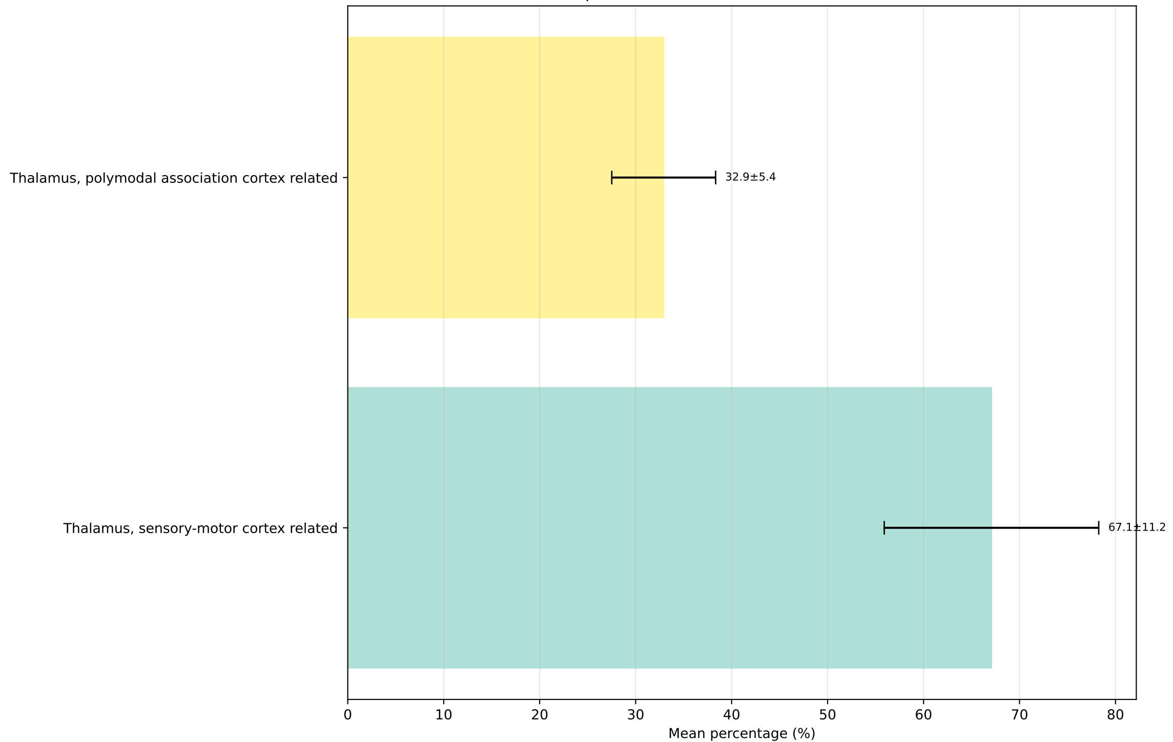
Thalamus: DORpm vs DORsm (Normalized to 100% within Thalamus)
