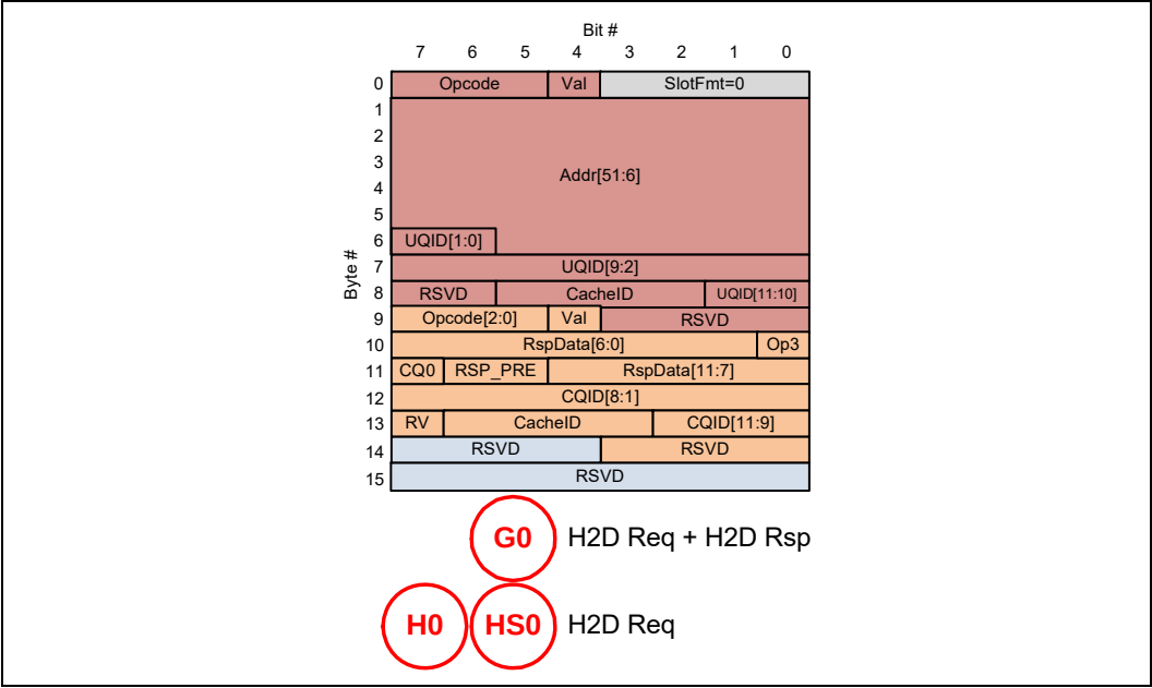
Figure 4-45. 256B Packing: G0/H0 PBR Messages
