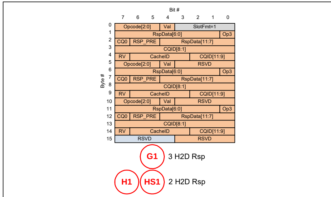
Figure 4-47. 256B Packing: G1/H1 PBR Messages
