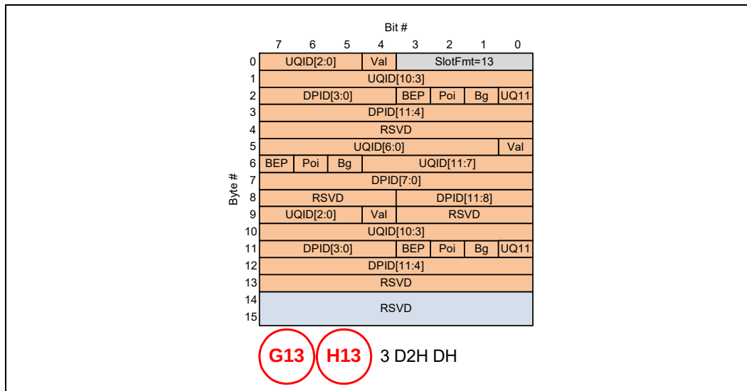
Figure 4-63. 256B Packing: G13/H13 PBR Messages
