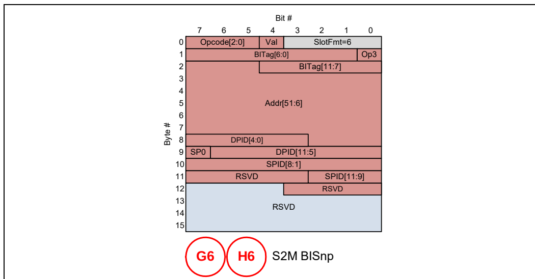
Figure 4-57. 256B Packing: G6/H6 PBR Messages
