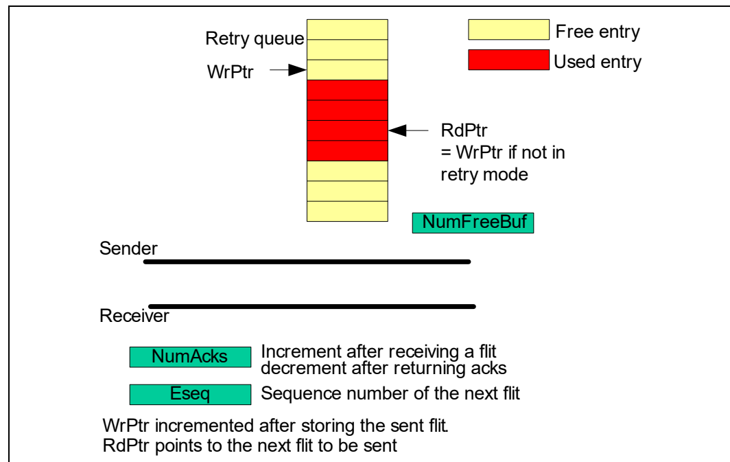
Figure 4-39. Retry Buffer and Related Pointers
