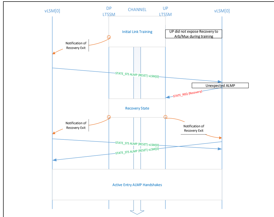
Figure 5-15. Upstream Port Hides Initial Recovery, Downstream Port Does Not
