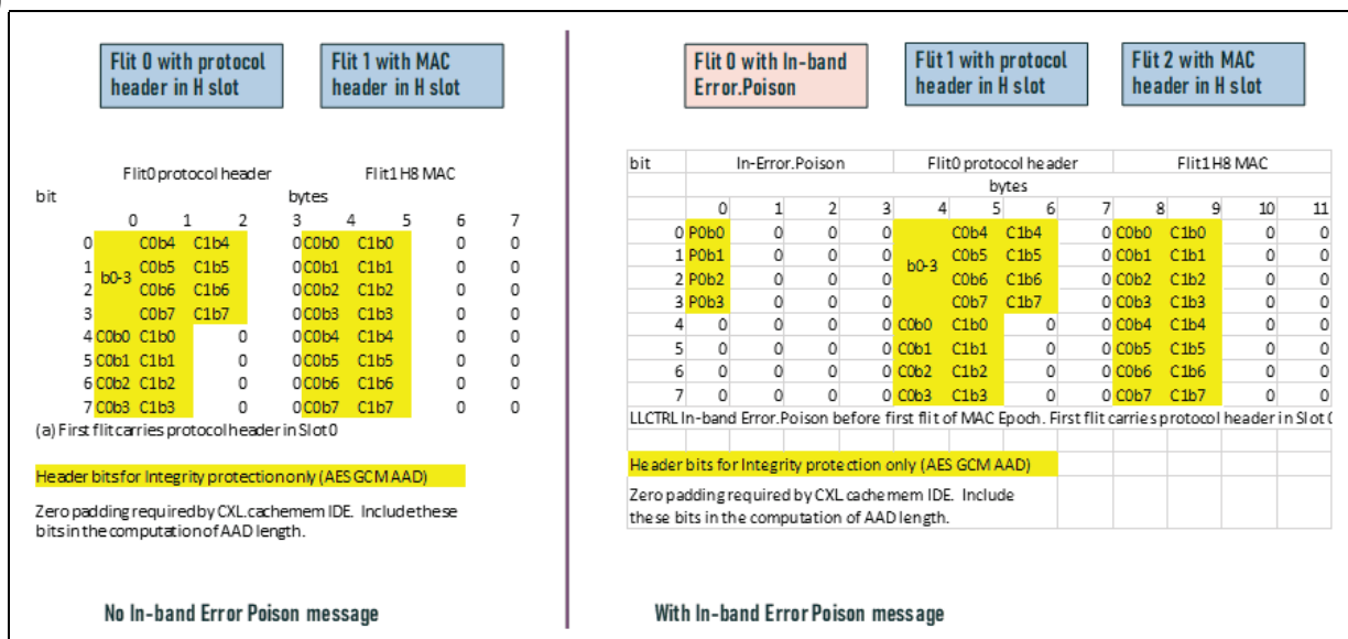
Figure 11-23. Containment Mode example illustrating the AAD construction for the case of two protocol flits that are part of the current MAC Epoch with an in-band LLCTRL Poison message sent after first flit of the MAC Epoch
