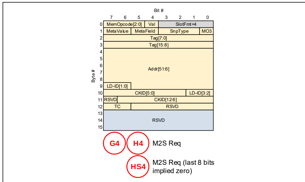
Figure 4-53. 256B Packing: G4/H4 PBR Messages
