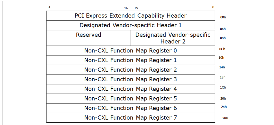
Figure 8-2. Non-CXL Function Map DVSEC
