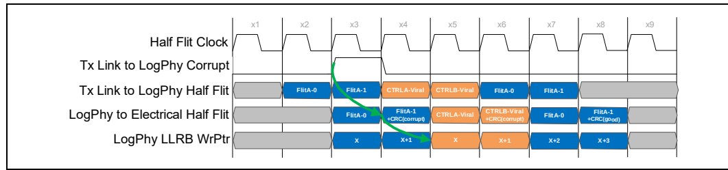
Figure 4-75. Viral Error Message Injection Standard 256B Flit
