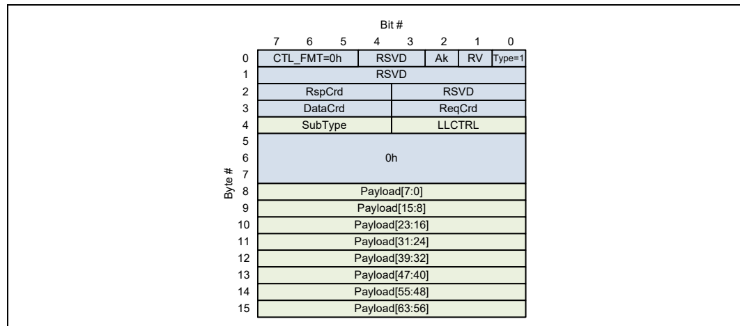
Figure 4-35. LLCRD Flit Format (Only Slot 0 is Valid; Others are Reserved)
