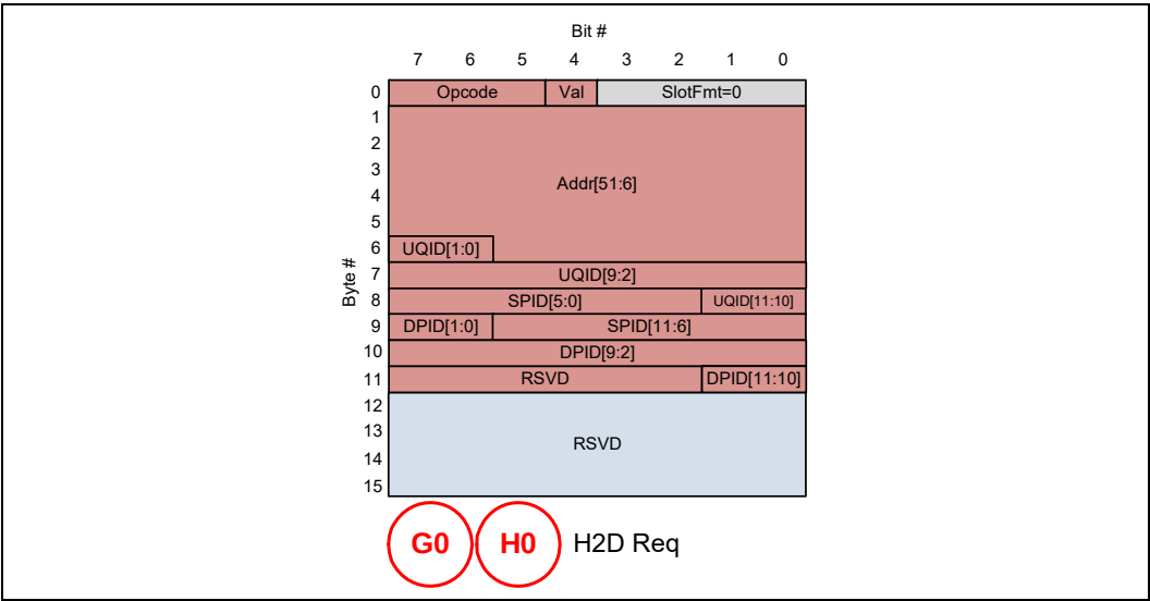
Figure 4-45. 256B Packing: G0/H0 PBR Messages
