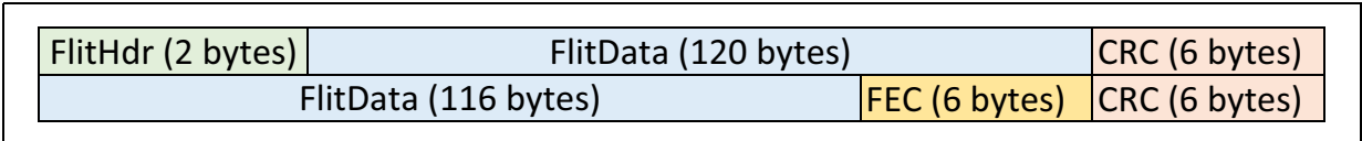
Figure 6-11. Latency-Optimized 256B Flit
