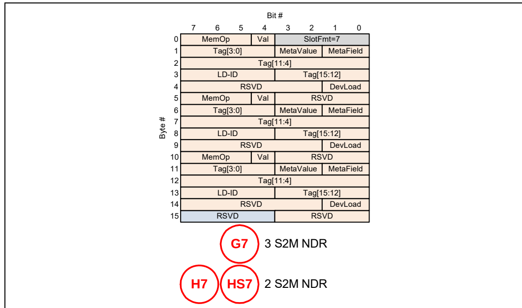
Figure 4-59. 256B Packing: G7/H7 PBR Messages
