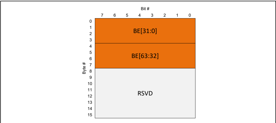
Figure 4-71. 256B Packing: Byte-Enable Trailer for D2H Data
