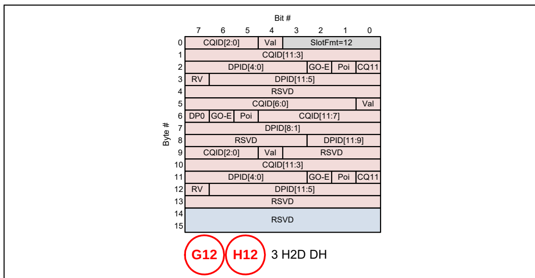
Figure 4-61. 256B Packing: G12/H12 PBR Messages
