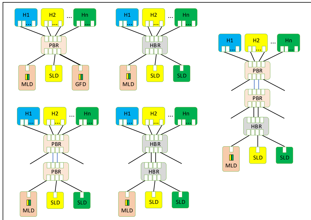
Figure 7-42. Example Supported Switch Configurations
