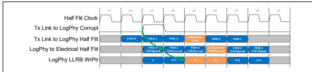
Figure 4-76. Viral Error Message Injection LOpt 256B Flit
