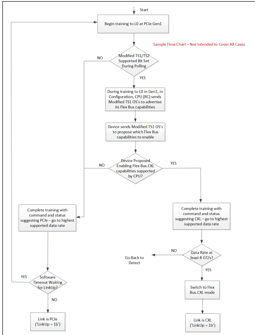
Figure 6-14. Flex Bus Mode Negotiation during Link Training (Sample Flow)
