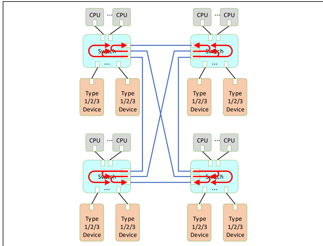
Figure 7-44. Example Routing Scheme for a Mesh Topology
