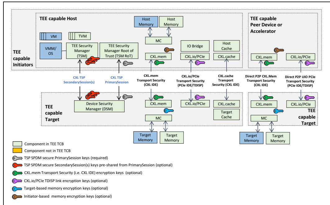
Figure 11-26. Reference Architecture
