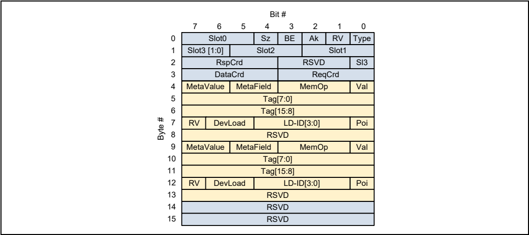
Figure 4-26. H6 - MAC
