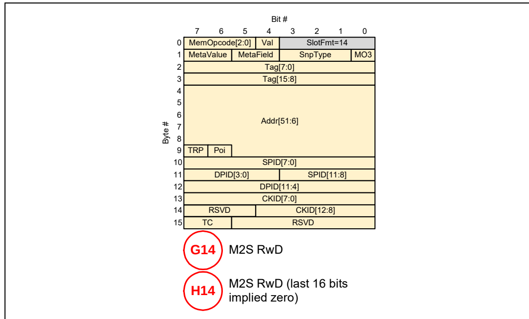
Figure 4-65. 256B Packing: G14/H14 PBR Messages
