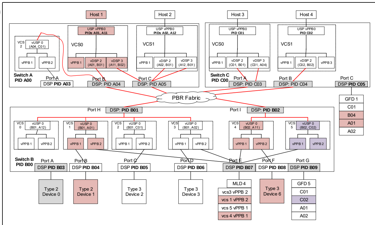
Figure 7-52. Single VH
