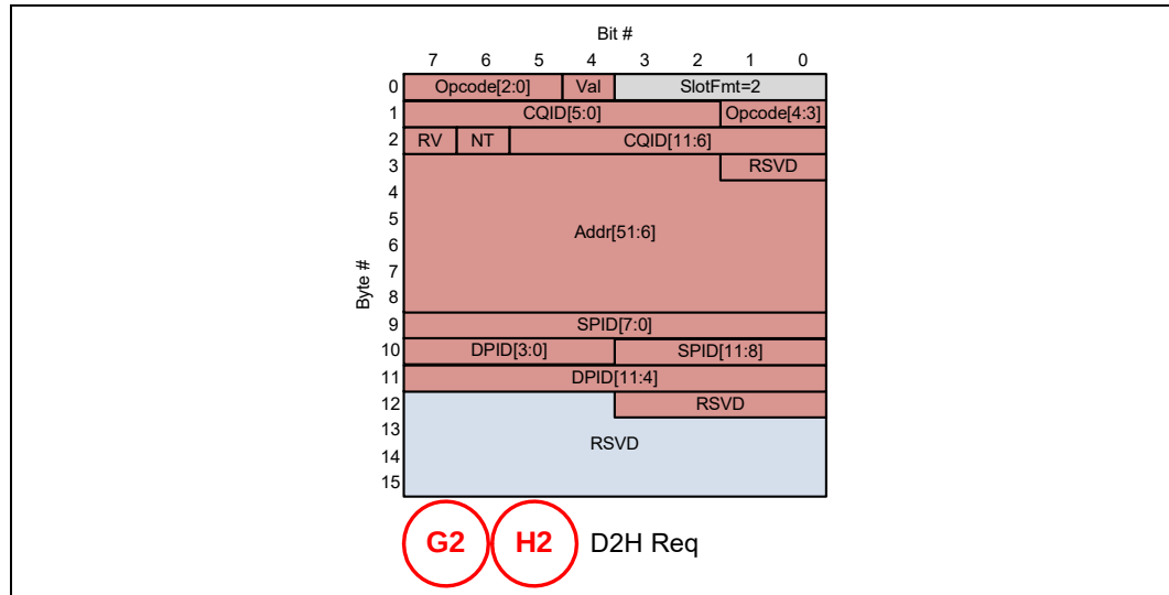
Figure 4-49. 256B Packing: G2/H2 PBR Messages
