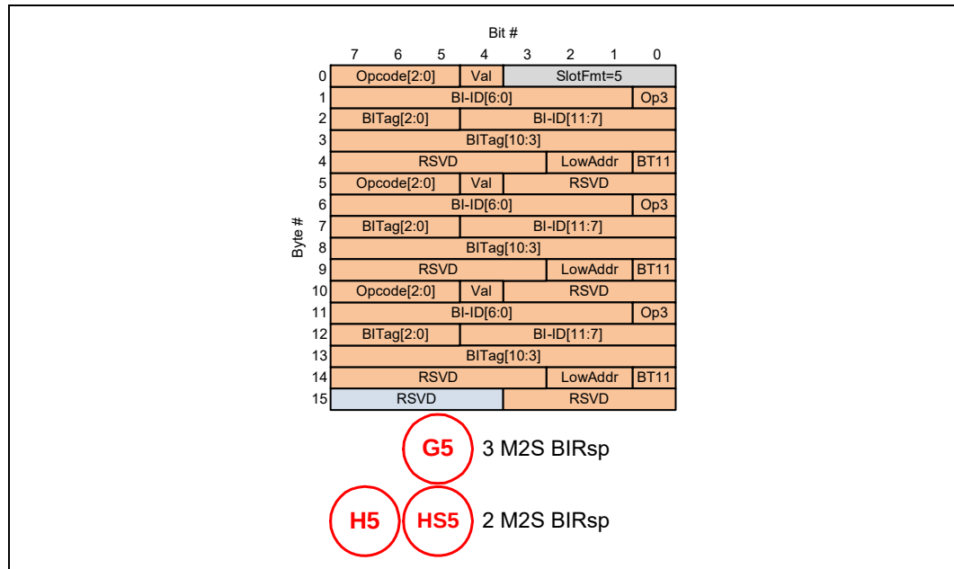
Figure 4-55. 256B Packing: G5/H5 PBR Messages
