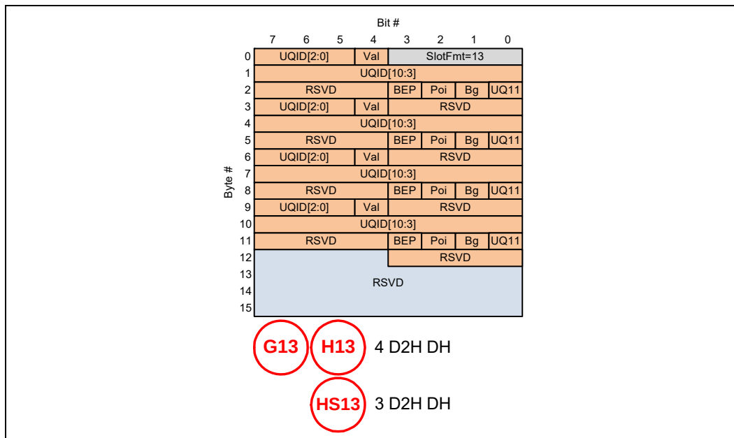
Figure 4-63. 256B Packing: G13/H13 PBR Messages
