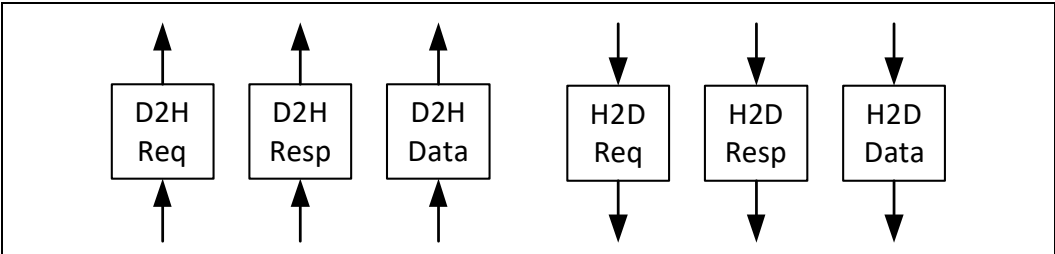
Figure 3-10. CXL.cache Channels
