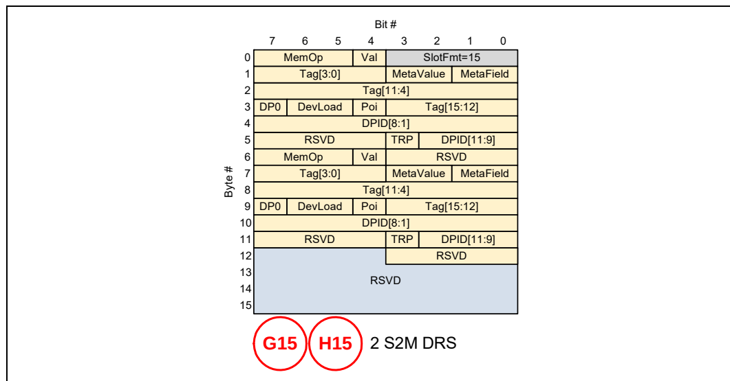
Figure 4-67. 256B Packing: G15/H15 PBR Messages
