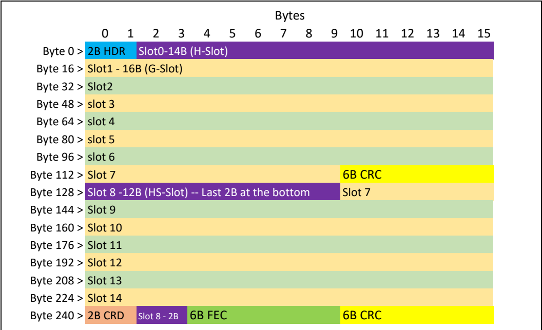
Figure 4-42. Latency-Optimized (LOpt) 256B Flit
