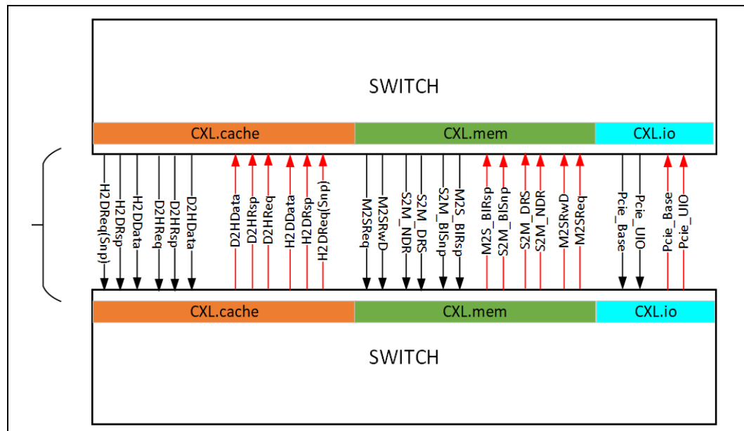
Figure 7-47. ISL Message Class Sub-channels
