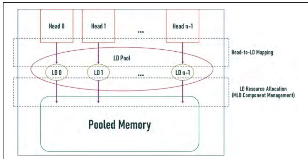
Figure 2-7. Head-to-LD Mapping in MH-SLDs
