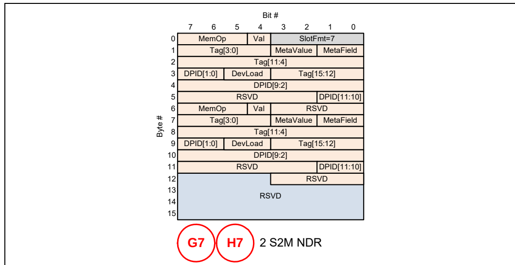
Figure 4-59. 256B Packing: G7/H7 PBR Messages
