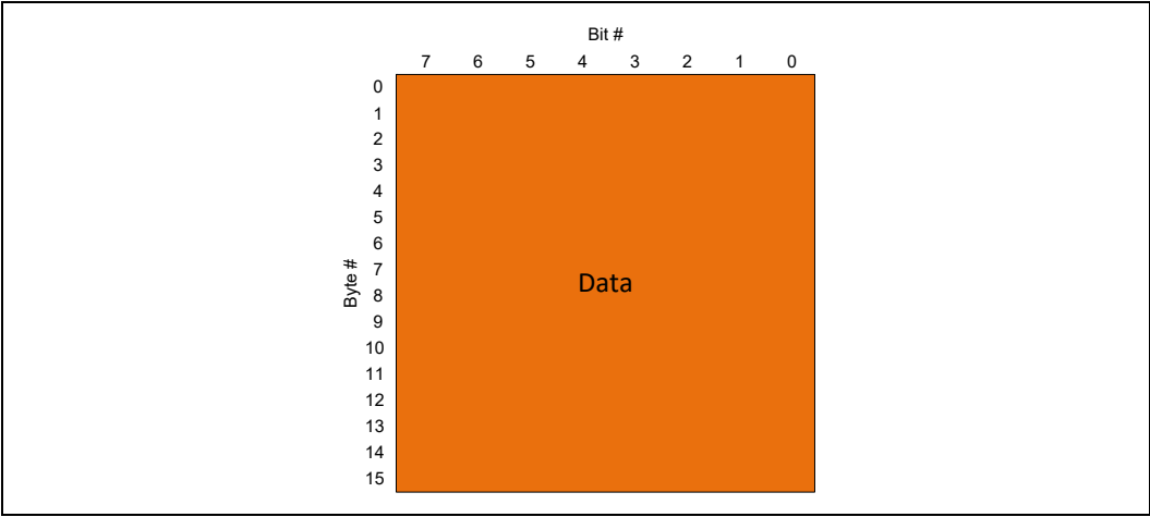
Figure 4-69. 256B Packing: Implicit Trailer RWD
