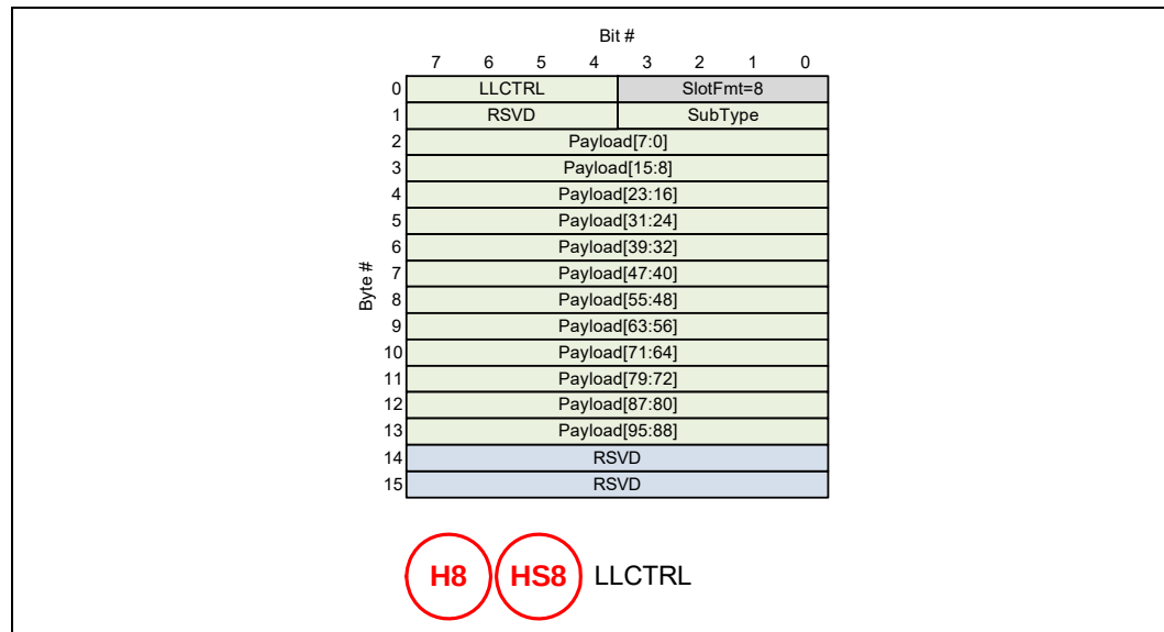
Figure 4-74. 256B Packing: H8/HS8 Link Layer Control Message Slot Format
