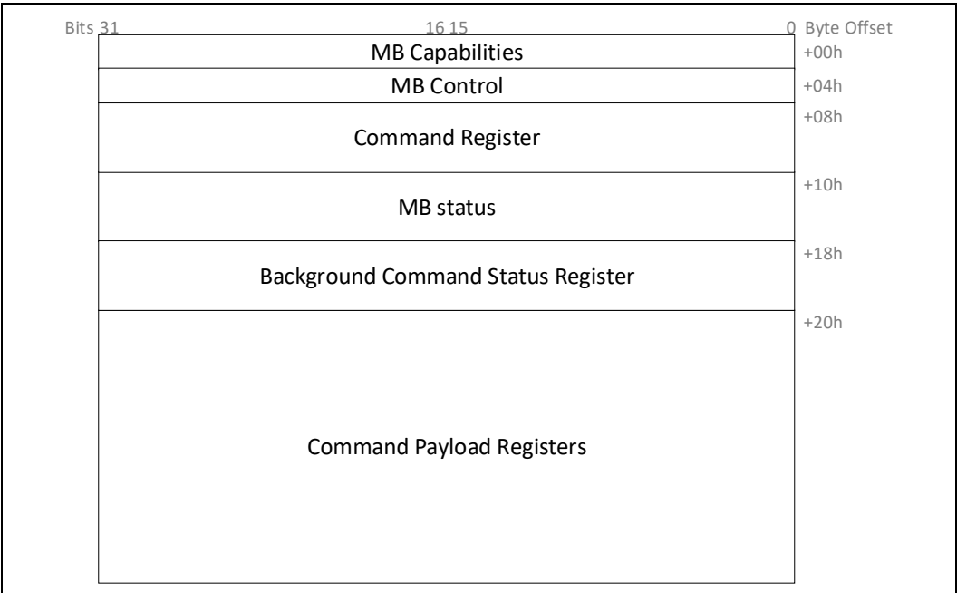
Figure 8-14. Mailbox Registers
