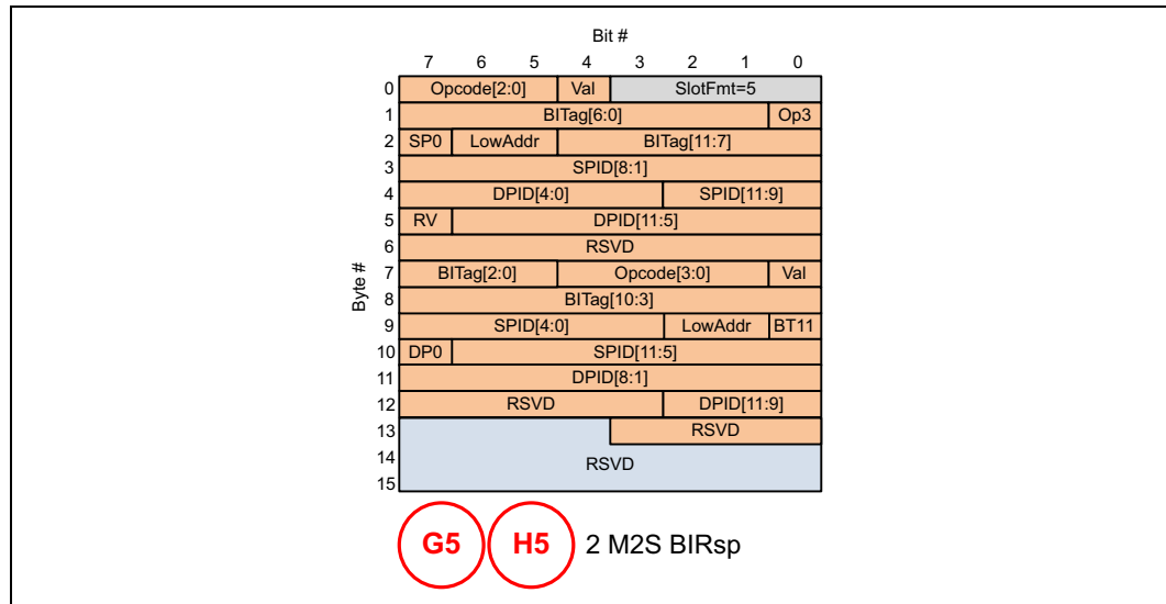
Figure 4-55. 256B Packing: G5/H5 PBR Messages
