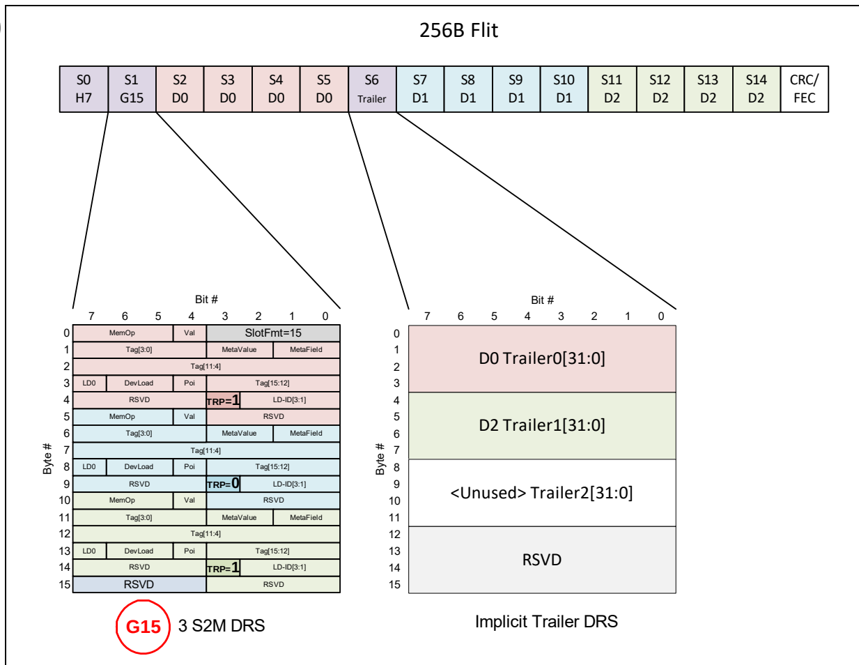
Figure 4-73. DRS Trailer Slot Decode Example
