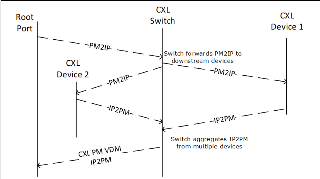
Figure 9-1. PMREQ/RESETPREP Propagation by CXL Switch
