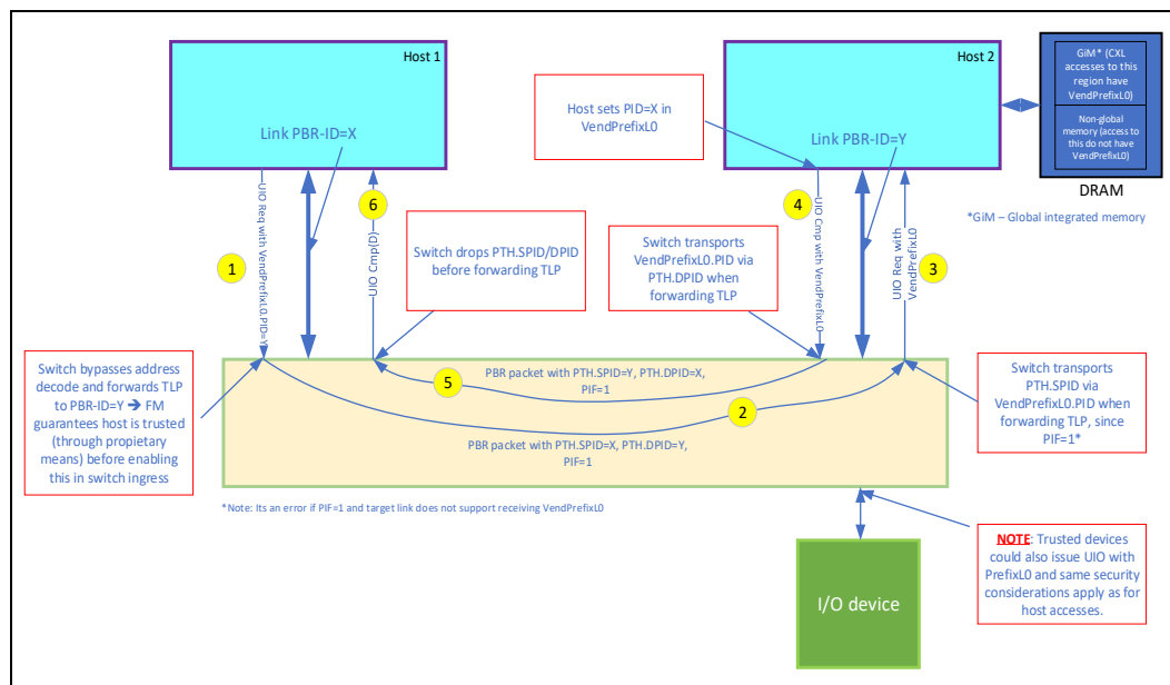
Figure 7-41. GIM Access Flows without FASTs
