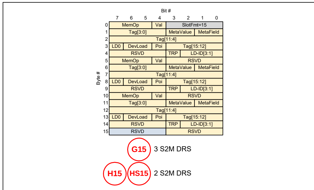
Figure 4-67. 256B Packing: G15/H15 PBR Messages
