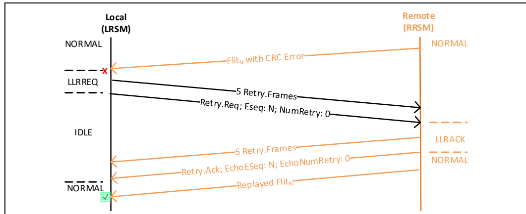
Figure 4-40. CXL.cachemem Replay Diagram
