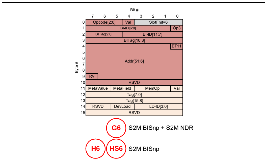
Figure 4-57. 256B Packing: G6/H6 PBR Messages
