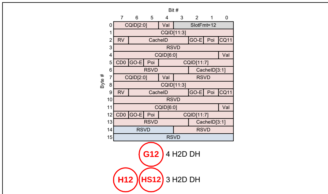
Figure 4-61. 256B Packing: G12/H12 PBR Messages
