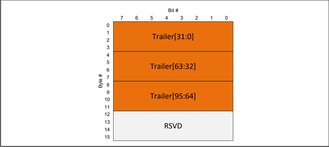
Figure 4-70. 256B Packing: Implicit Trailer DRS
