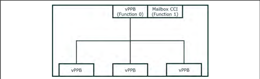
Figure 7-15. Multi-function Upstream vPPB
