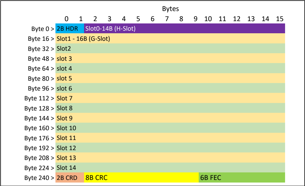
Figure 4-41. Standard 256B Flit
