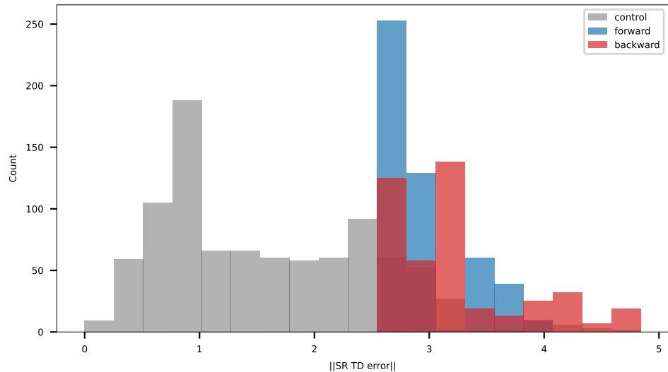
Pooled teleport TD-error norm across sessions
