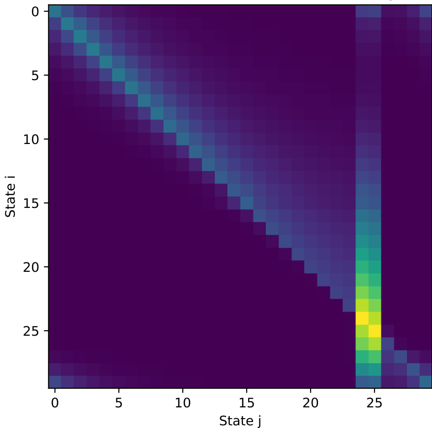
SR matrix reward location switch - Early
