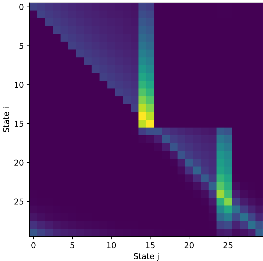
SR matrix reward location switch - Late
