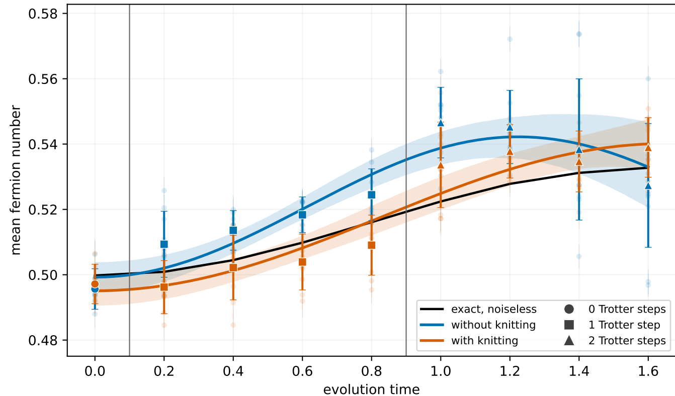
Time Evolution of Mean Fermion Number
