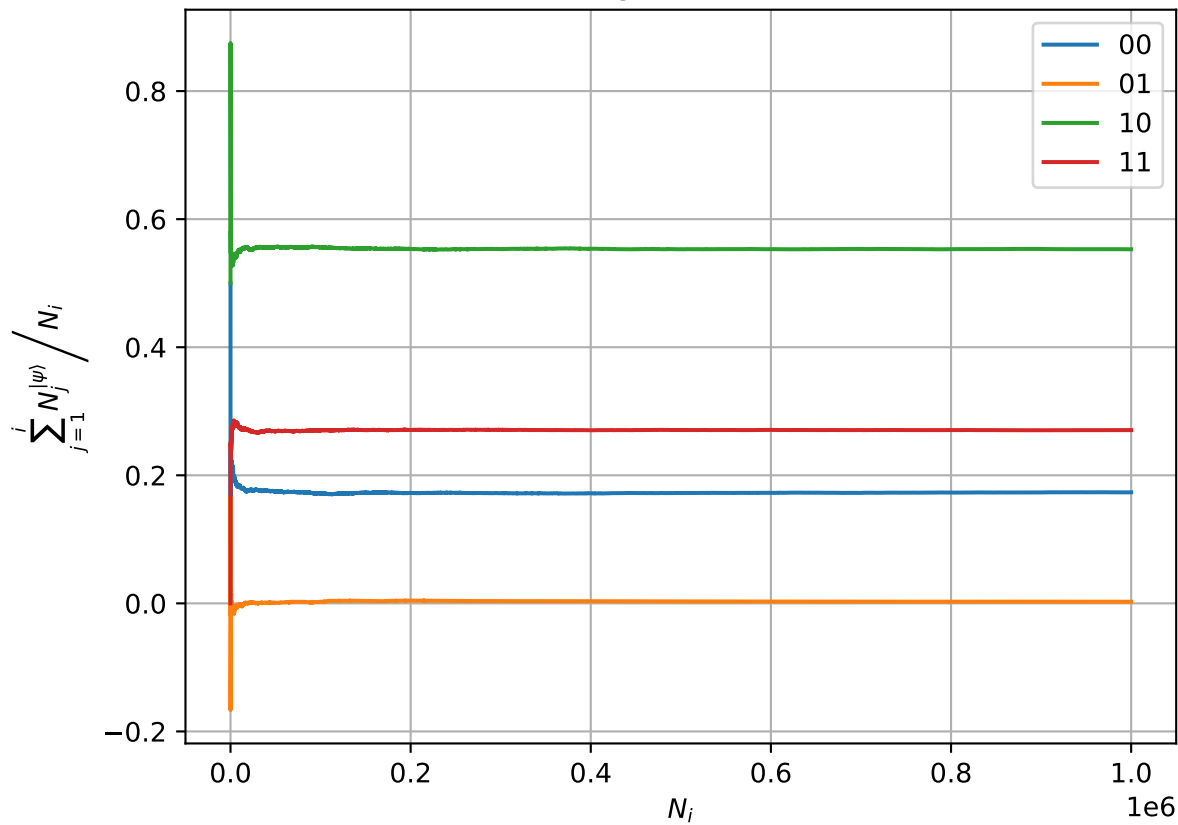
Convergence of Ratios
