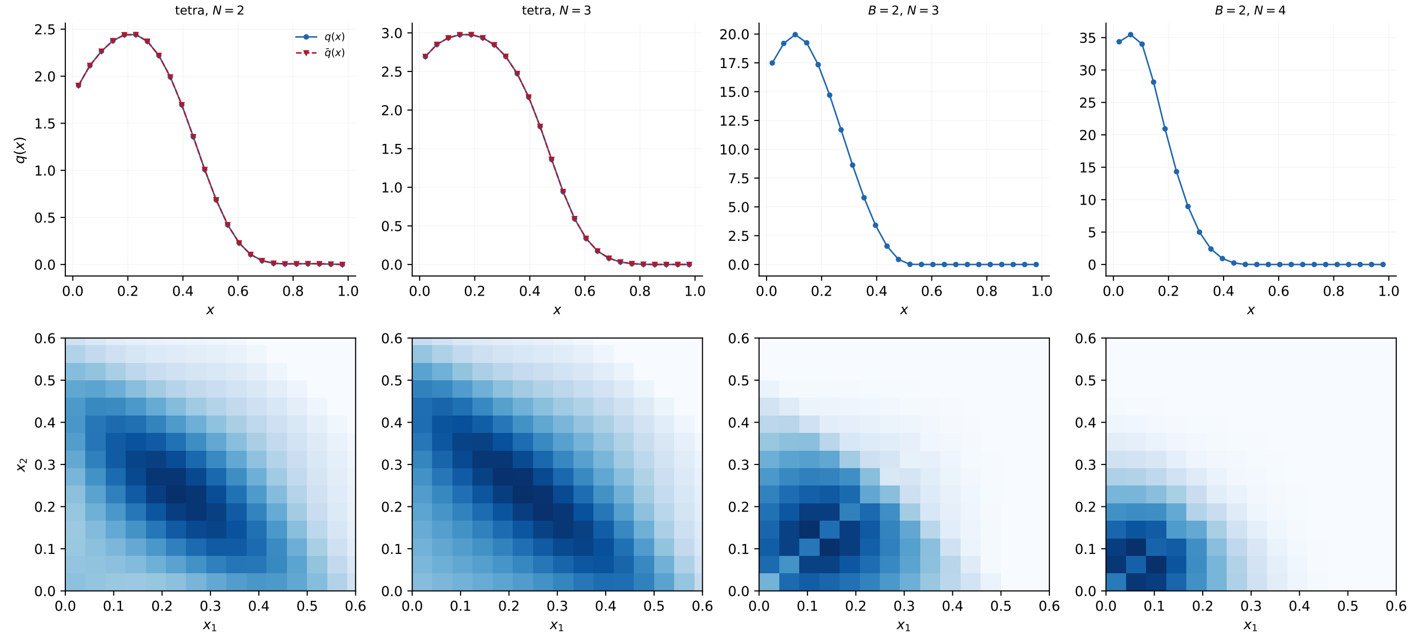
FIG. 10: the exotic candidates at m/g = 0.1 , 2K = 48 , standard Hamiltonian, dominant Fock sectors; top q(x) , bottom the pair correlation C(x_1, x_2)
