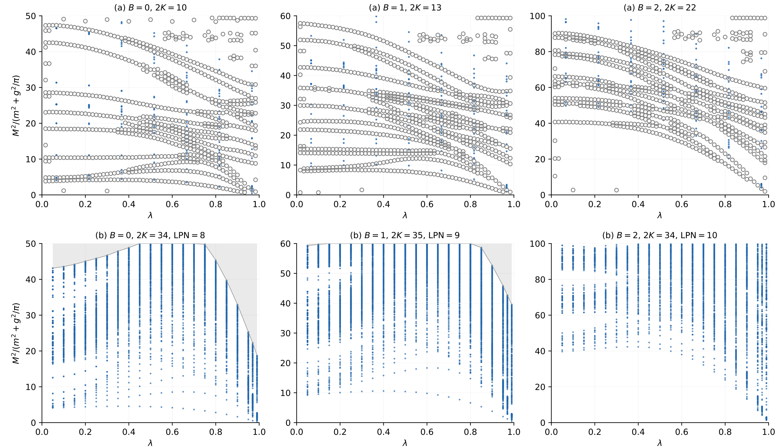
FIG. 2: spectra vs coupling — 1990 reproduction (top, markers digitized from HBP) and 2026 (bottom)
