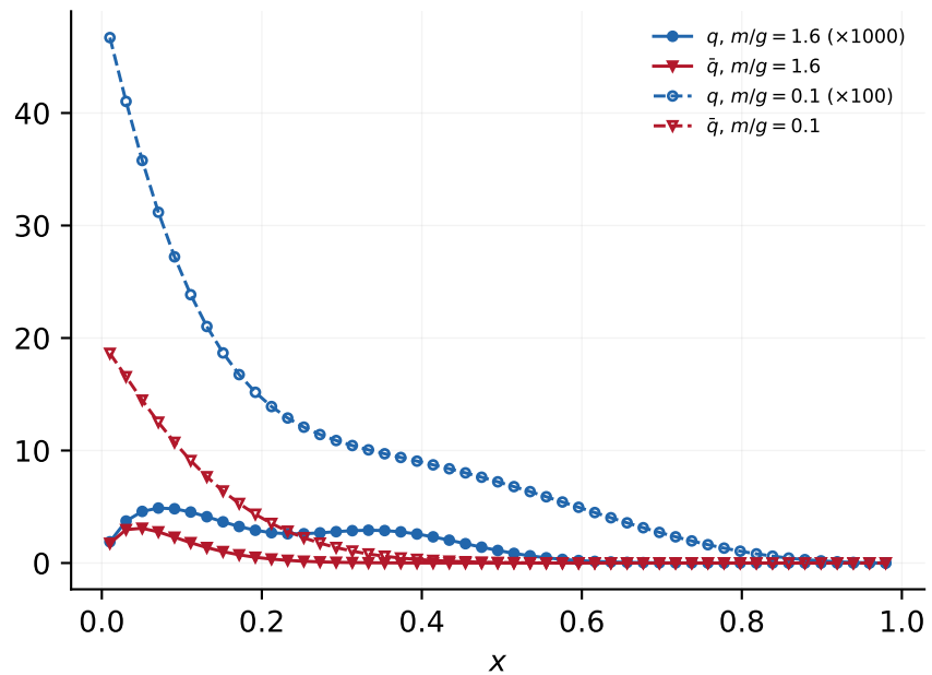
(b) baryon 5q, 2K = 99 , LPN = 5
