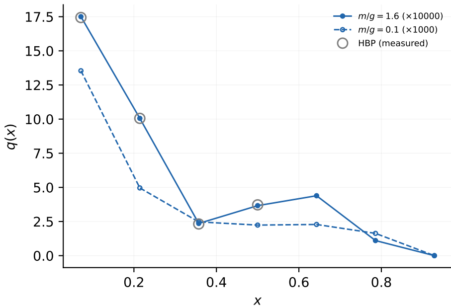
(b) meson 4q, 2K = 100 , LPN = 6
