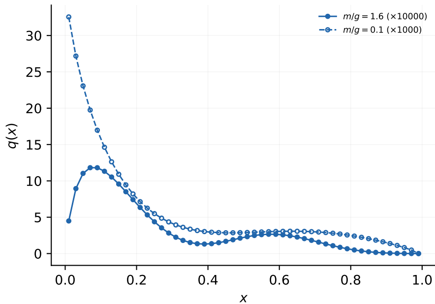
(b) meson 4q, 2K = 100 , LPN = 6
