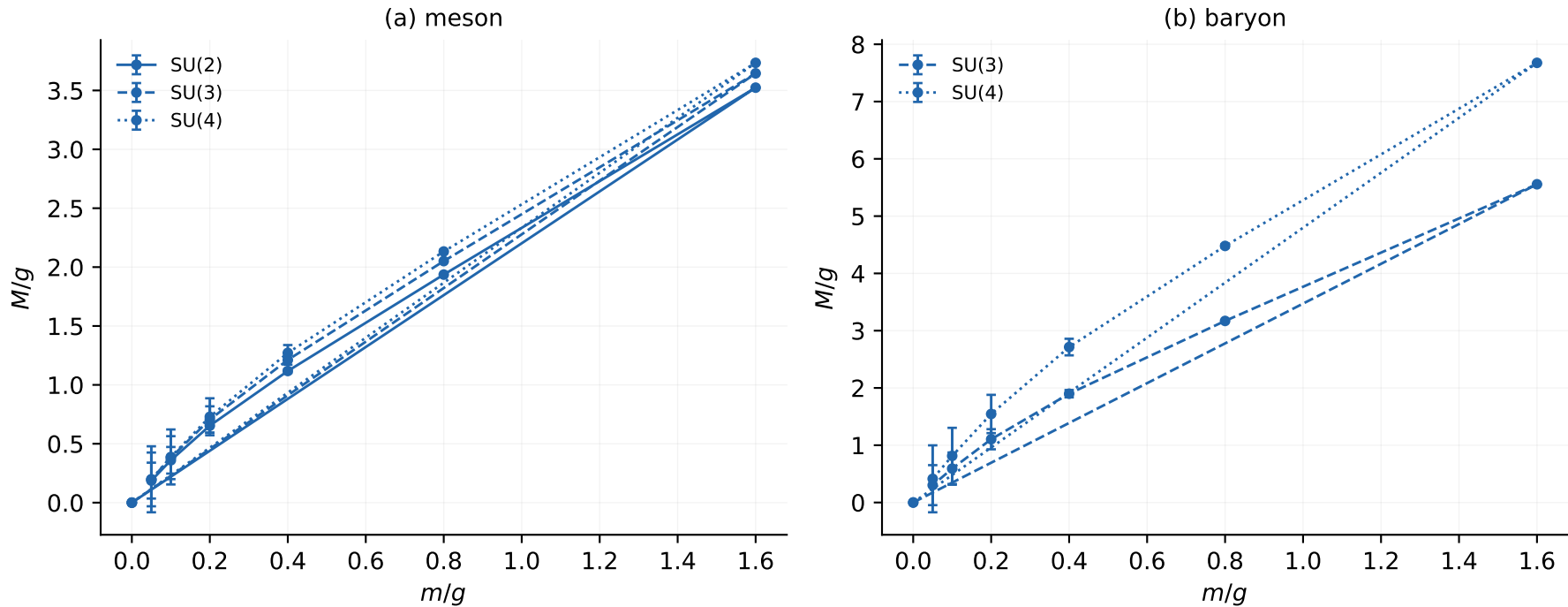
FIG. 7: extrapolated masses, standard Hamiltonian, Eq.~(27) fits over 2K = 25\text{--}71 , full budget bars
