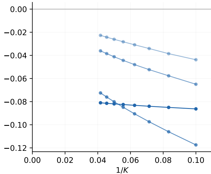
(b) tetraquark channel, N = 3
