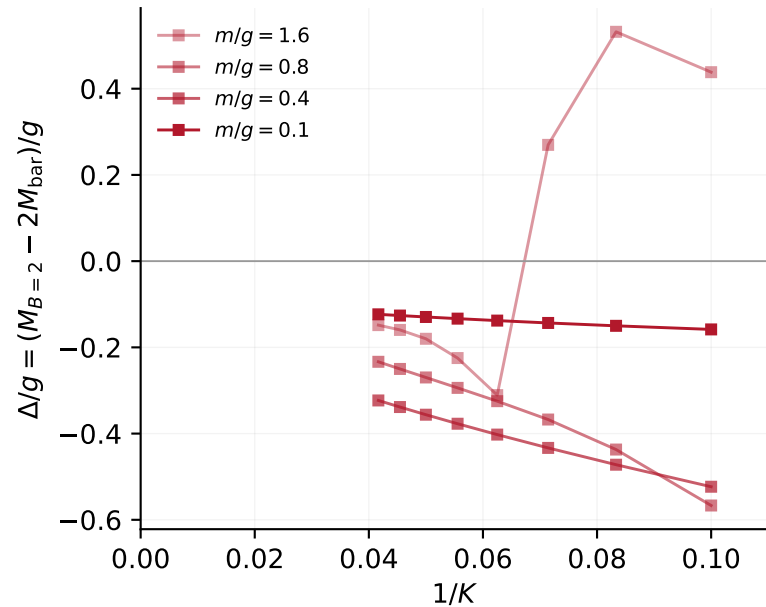
(c) two-baryon channel, N = 4
