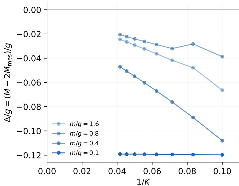
(a) tetraquark channel, N = 2
