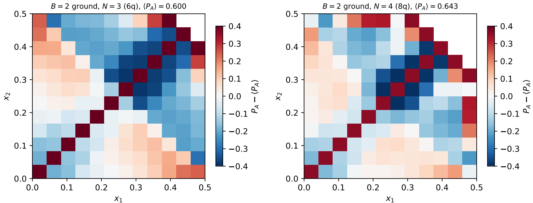
FIG. 11: antitriplet (diquark-channel) probability of quark pairs, m/g = 0.1 , 2K = 48 , standard Hamiltonian, valence sectors
