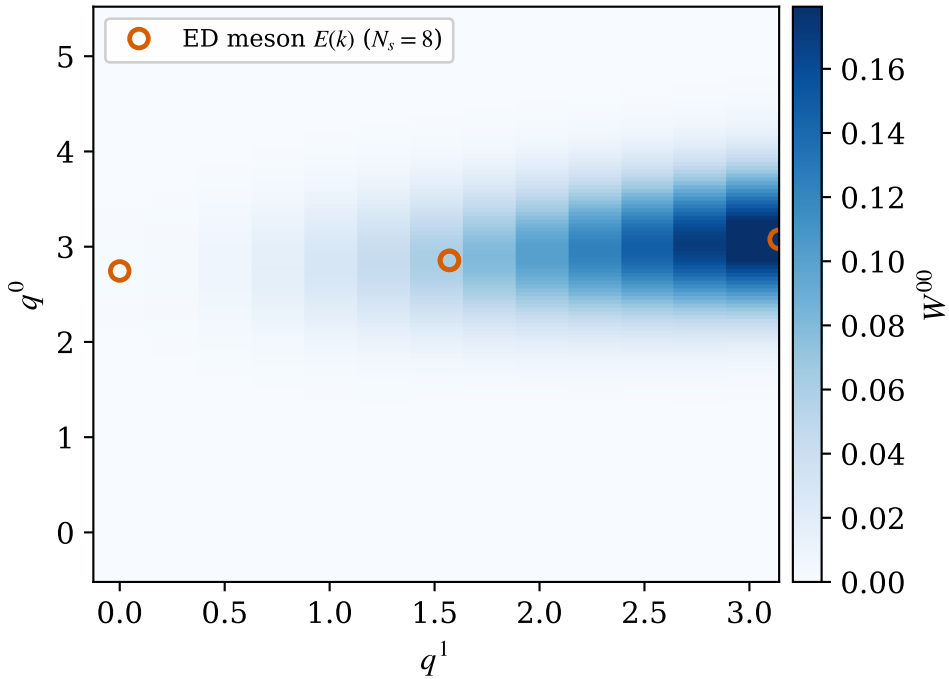
W_{\text{vac}}^{00}(q^0, q^1) , N_s = 50 (101 qubits, MPS)
