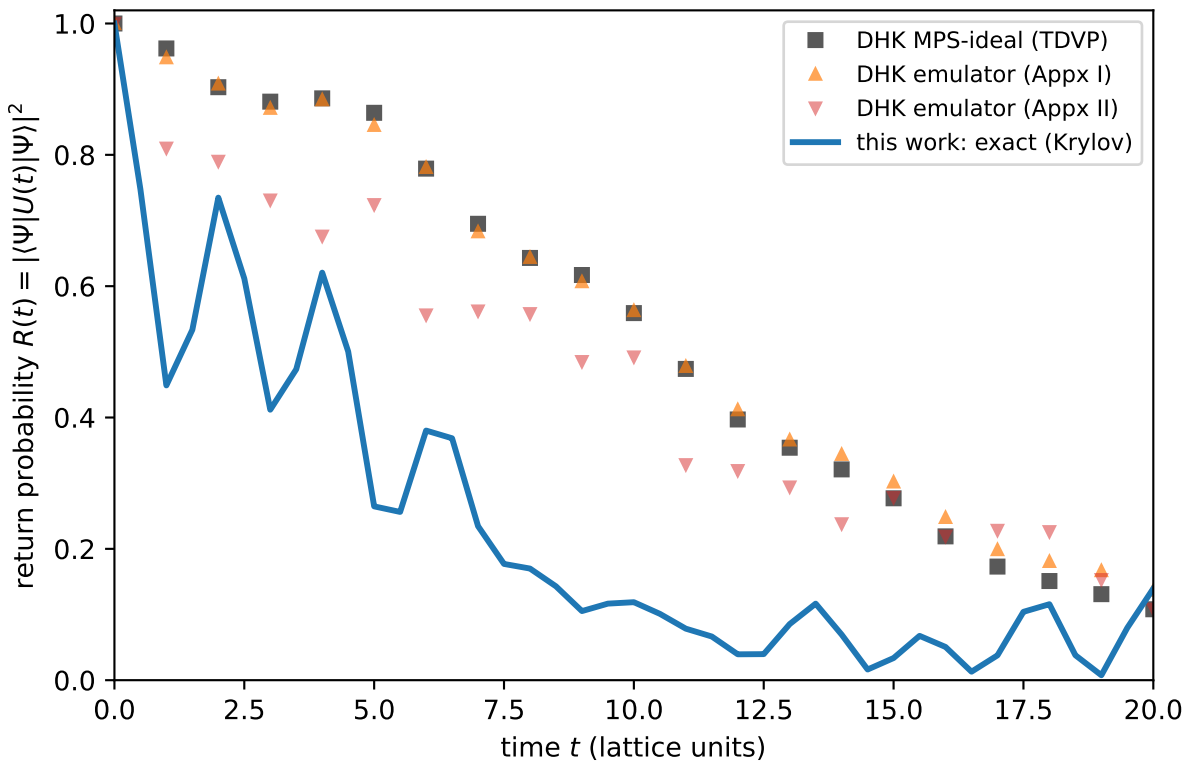
DHK N_p = 13 meson-meson collision: exact vs approximate
