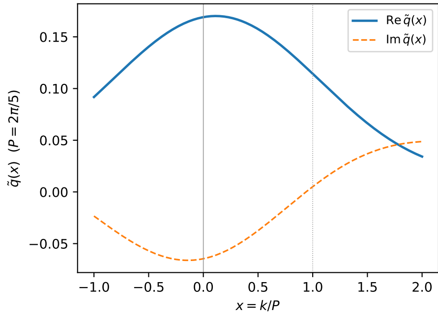
Quasi-PDF from the 101-qubit boosted meson (equal-time, no ancilla)
