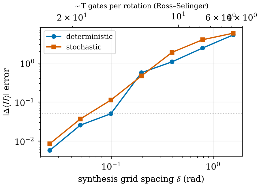
Physics vs rotation-synthesis error ( N_s = 8 pilot, full pipeline)
