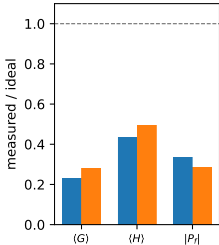
(b) global certificates
