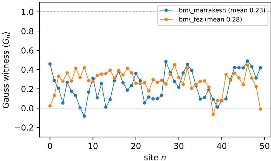
(a) gauge-law stabilizers, 101 qubits
