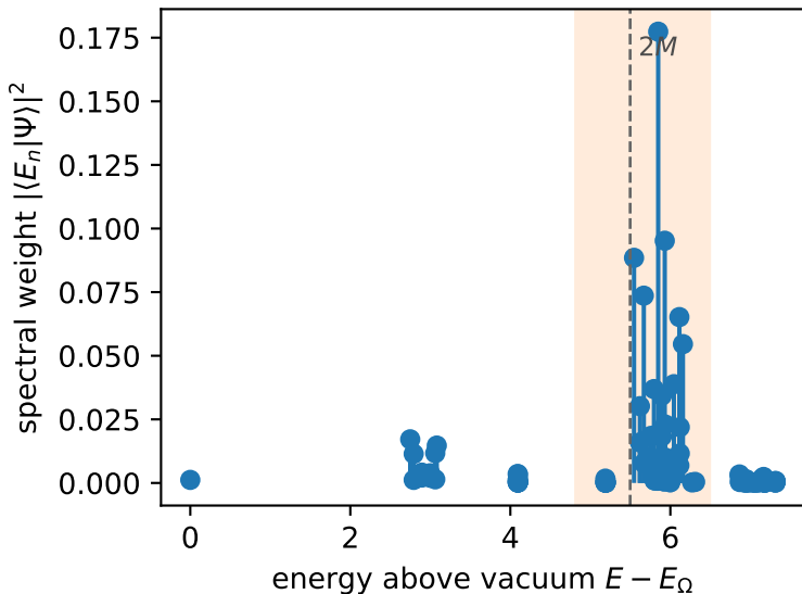
our prepared state ( N_P = 5 ): \sigma_E = 0.84
