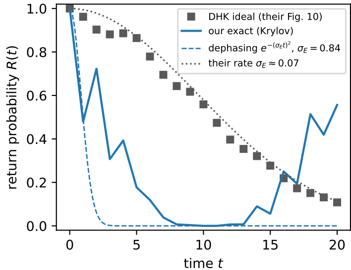
R(t) at their production volume ( N_P = 13 )
