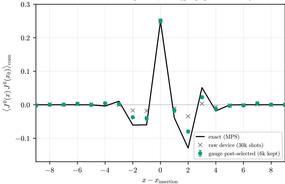
Connected screening cloud, t = 0 (gauge post-selection)
