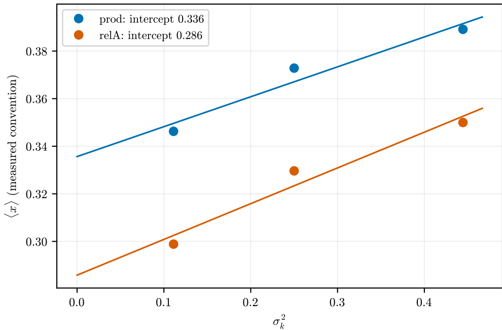
quasi-PDF width scan, classical references (Ns=50 preps)
