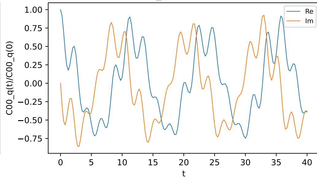
C00_q, P = +0.628
