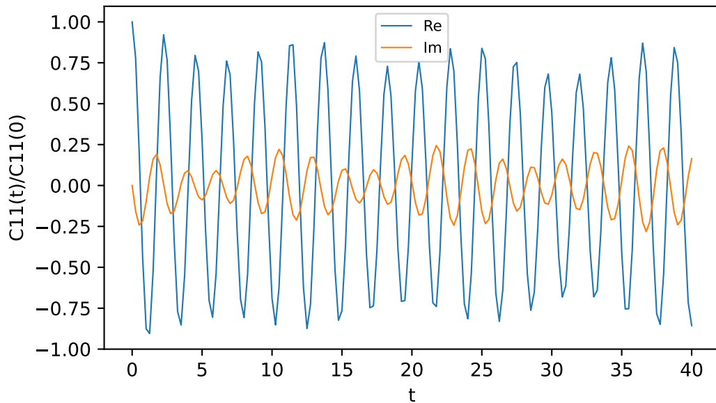
C11, P = +0.000
