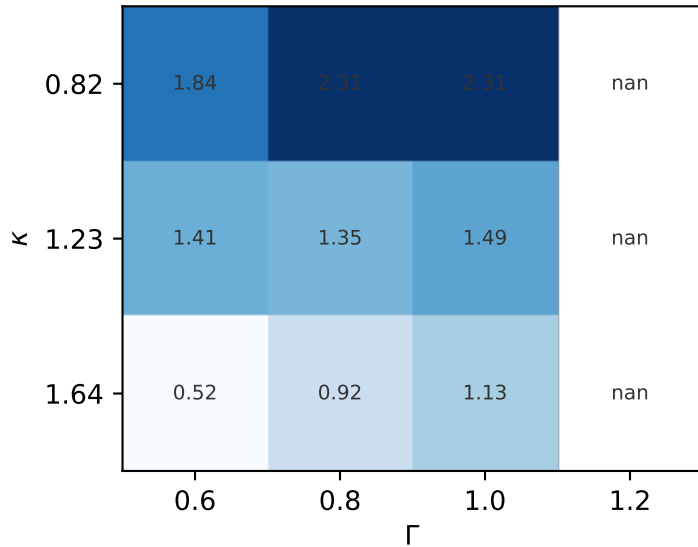
(a) baryon/meson [%]
