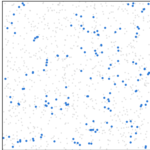
t = 56 \text{ fm}/c ( L = 76 \text{ fm} )
