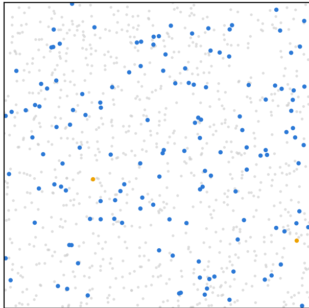
t = 1 \text{ fm}/c ( L = 13 \text{ fm} )
