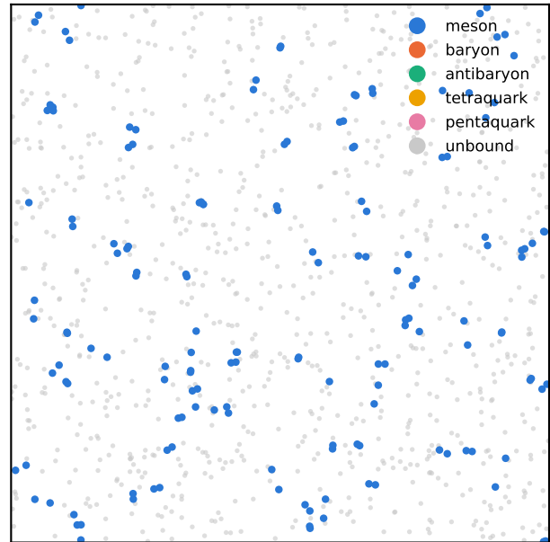
t = 110 \text{ fm}/c ( L = 138 \text{ fm} )
