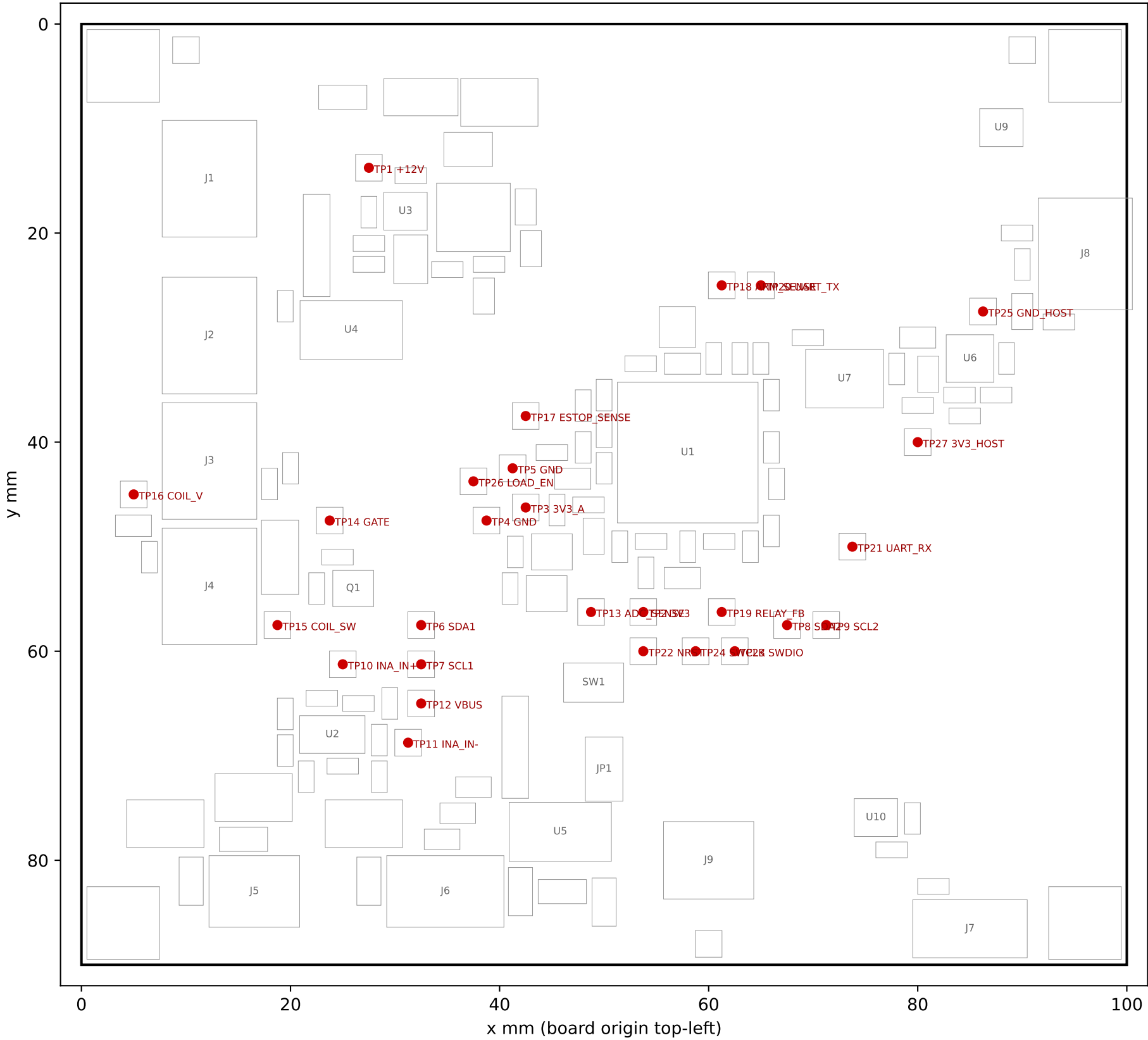
OSBAMS Rev.2 Controller - test-point map (27 points) RC1.2 - REVIEW CANDIDATE - NOT RELEASED FOR FABRICATION
