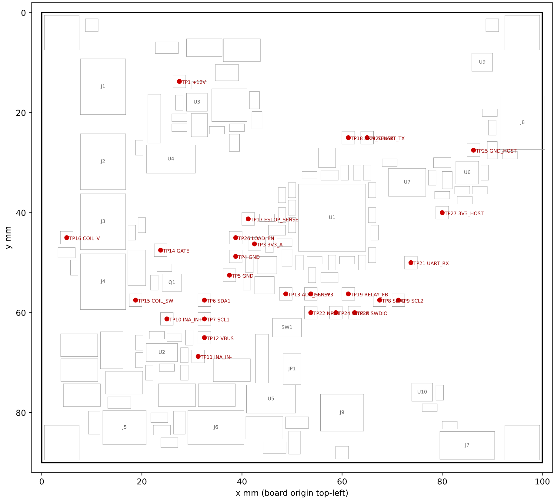
OSBAMS Rev.2 Controller - test-point map (27 points) RC1.3 - REVIEW CANDIDATE - NOT RELEASED FOR FABRICATION
