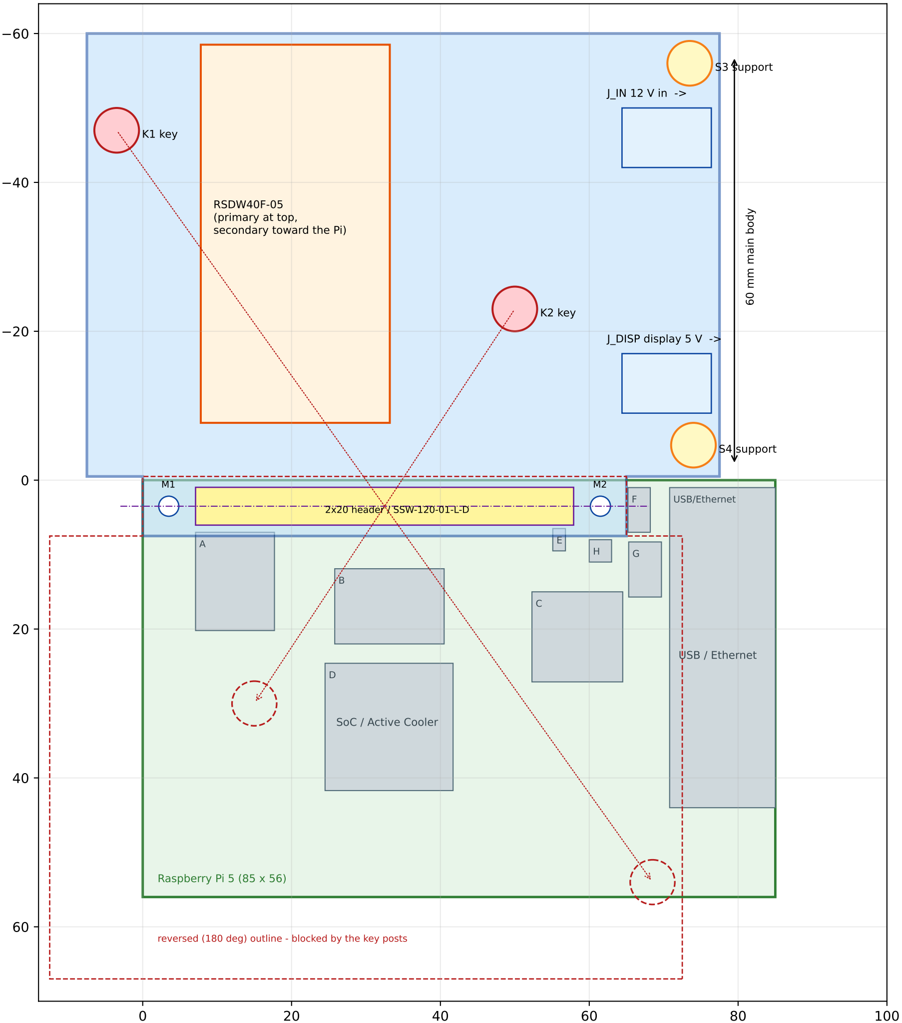
OSBAMS Pi Power Carrier RevB - mechanical placement over the Raspberry Pi 5 (plan view, Pi frame, mm)
