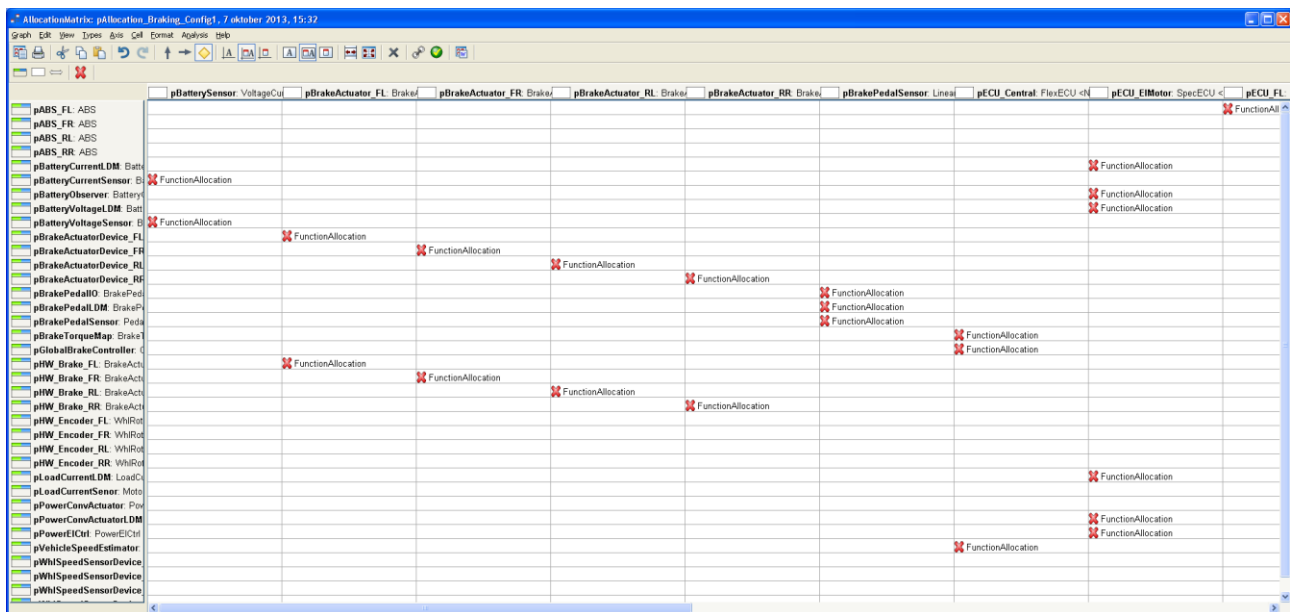
Figure 13. Example of EAST-ADL Function-to-Node allocation
