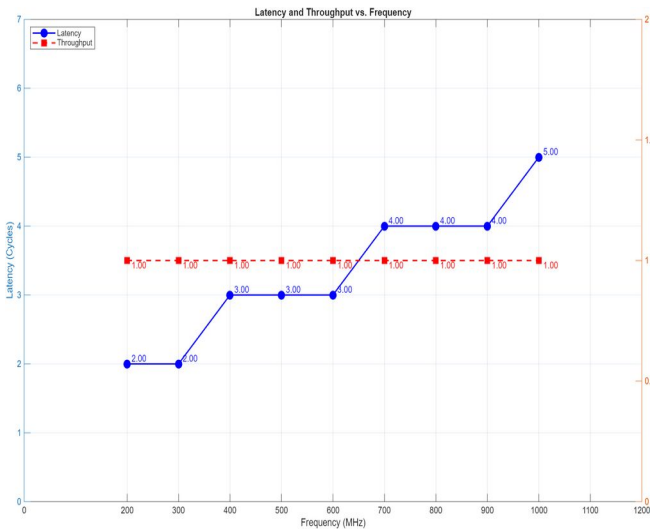
Throughput vs Frequency
