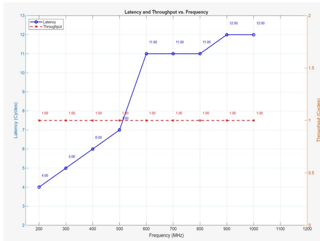
Throughput vs Frequency
