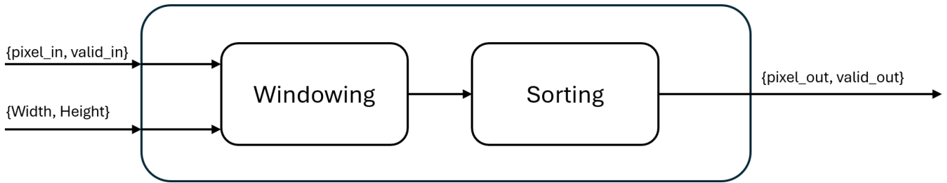
Fig. 1: Block diagram of Median2D Filter.
