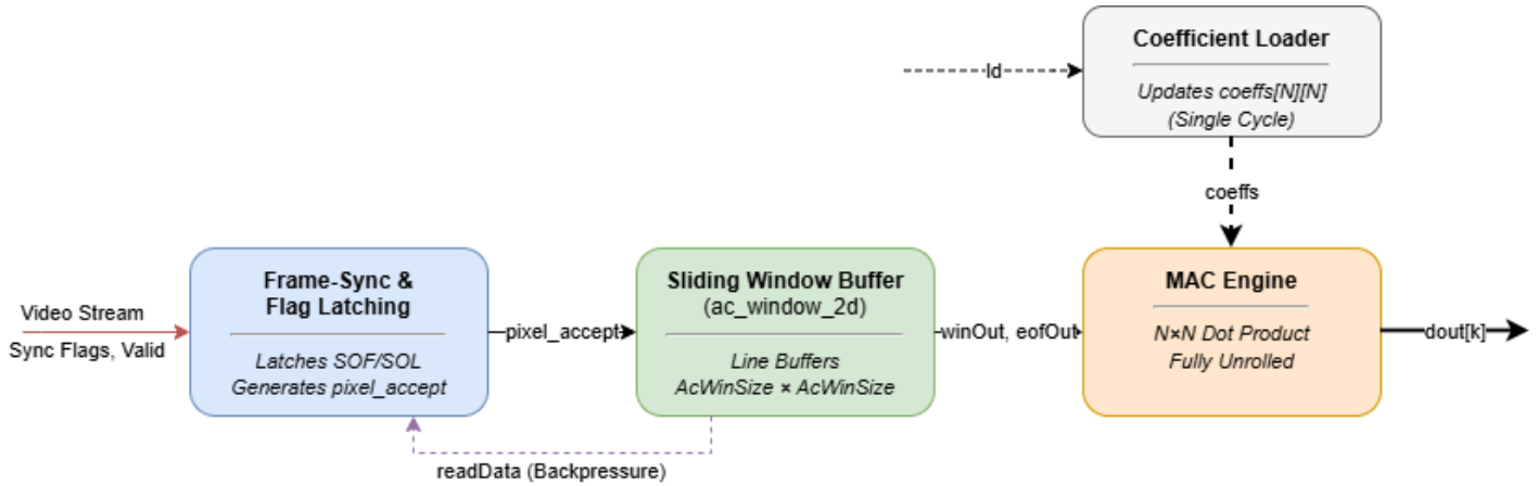
Illustration 37: Block Diagram
