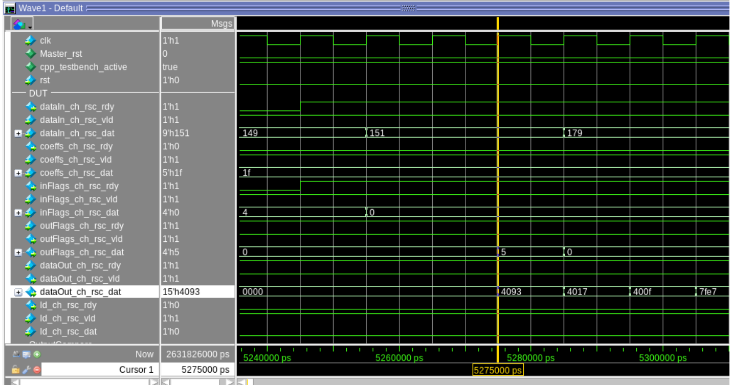
Illustration 40: RTL waveform
