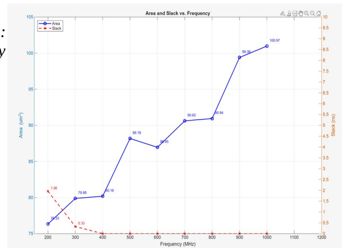
Fig. 4: Area and Slack vs Frequency
