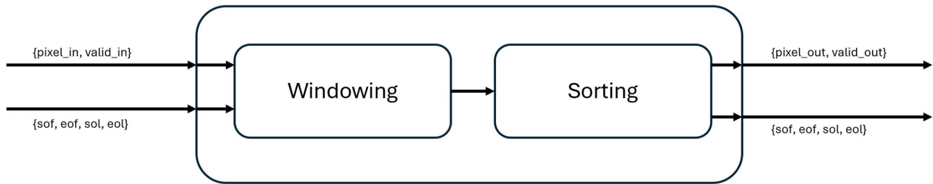
Fig. 1: Block diagram of Median2D Filter with sync flags.
