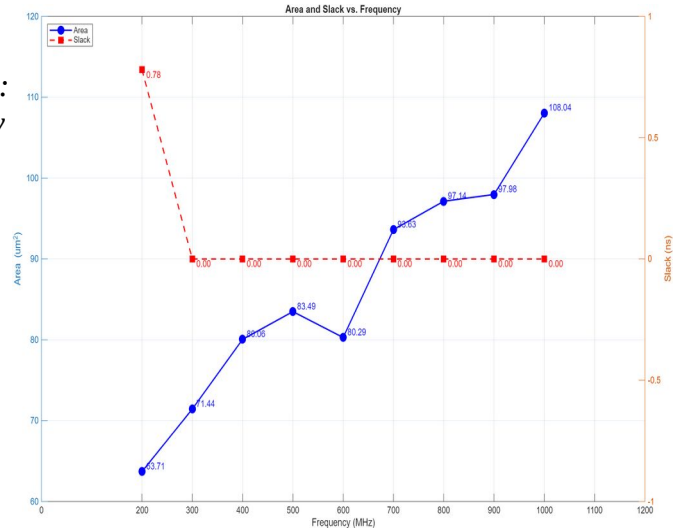
Fig. 4: Area and Slack vs Frequency
