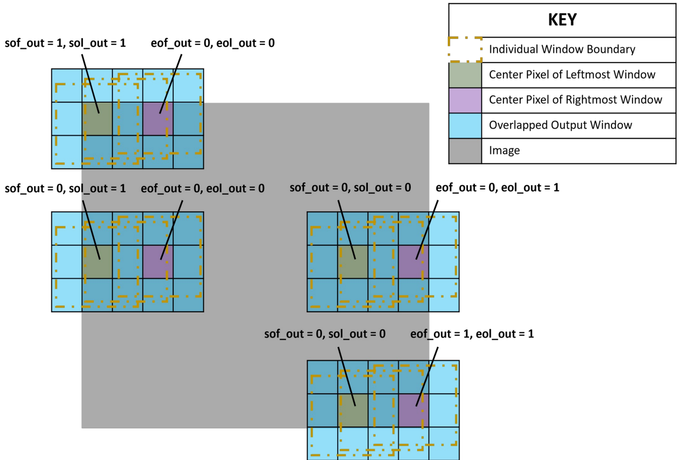
Illustration 50: Output Flags for Different Window Positions, with Boundary Padding
