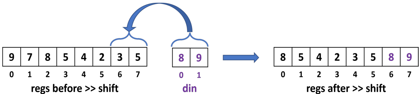
Illustration 42: Right-shifting Data Values
