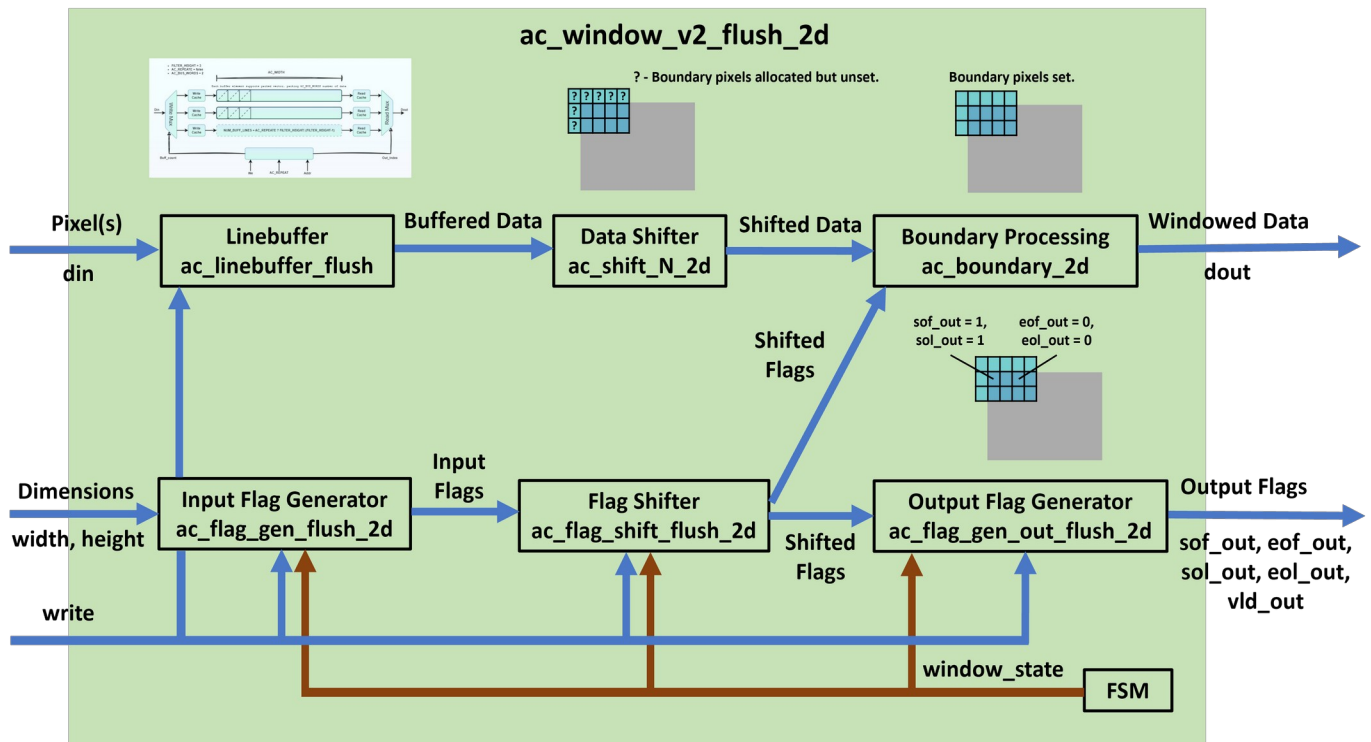
Illustration 54: Block Diagram for Flushing Support
