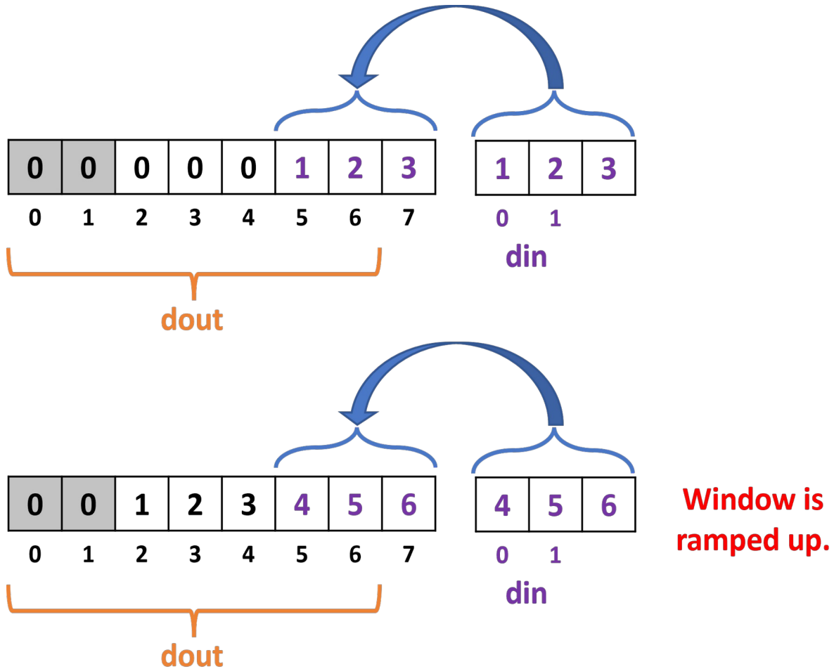
Illustration 47: Horizontal Window Rampup
