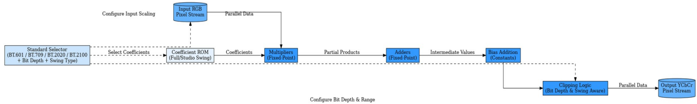
Illustration 4: Block diagram for Color Space Conversion design
