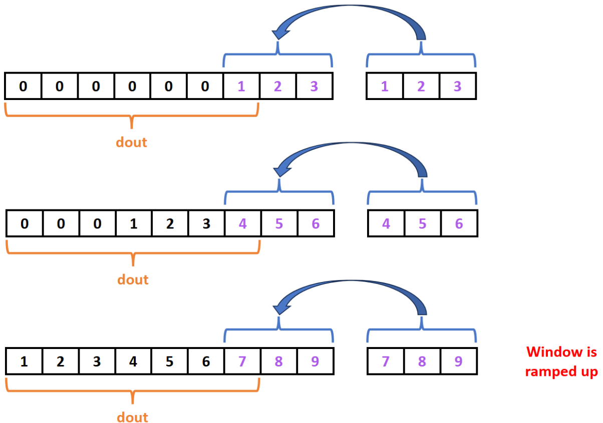
Illustration 48: Horizontal Window Rampup, without Padding
