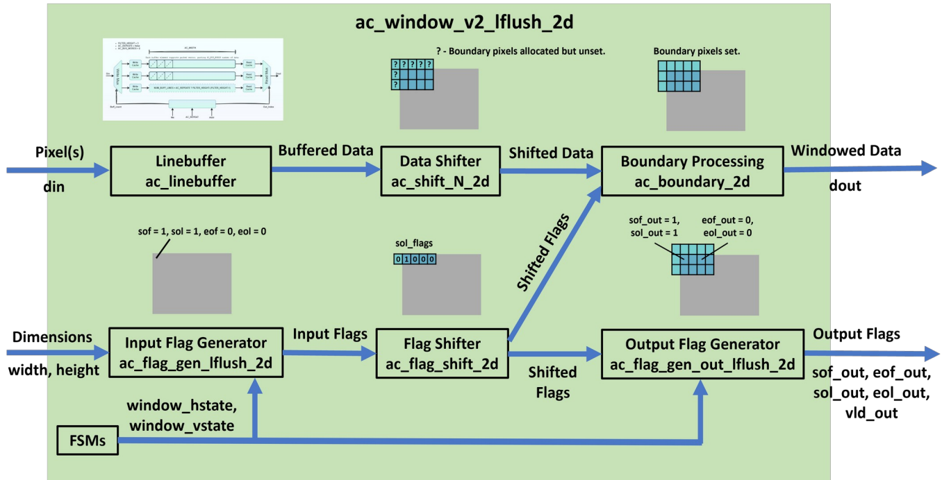
Illustration 55: Block Diagram for Line Flushing
