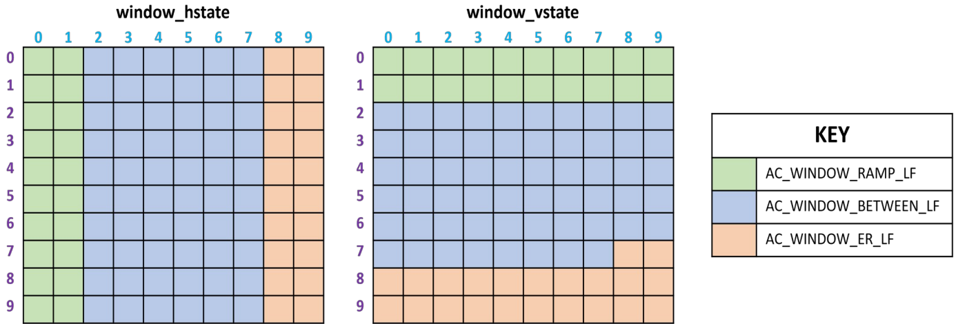
Illustration 57: window_hstate and window_vstate Values in Different Image Regions
