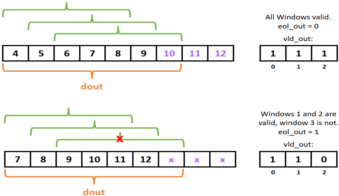
Illustration 51: vld_out Generation at EOL, without Padding
