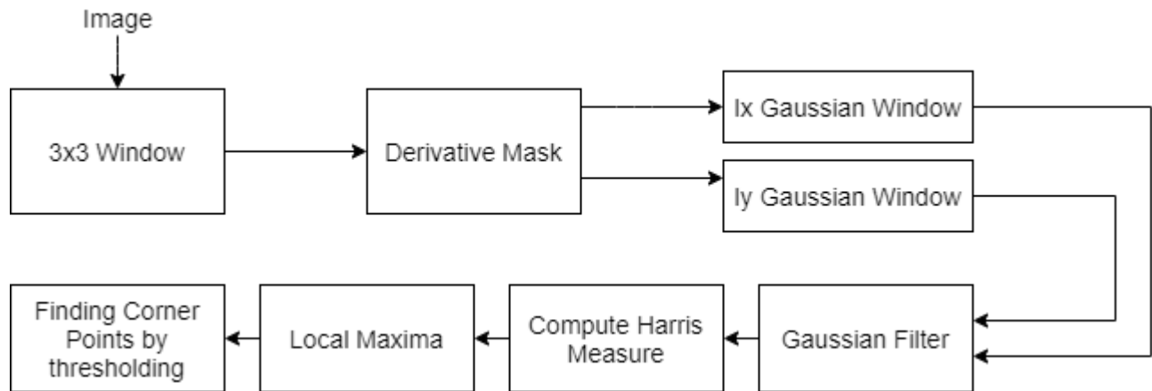
Illustration 26: Harris Corner Detector Block Diagram
