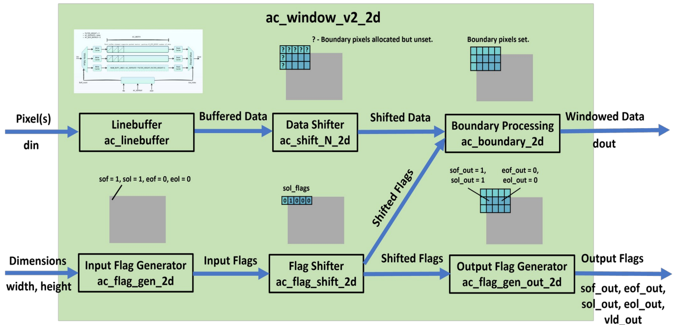
Illustration 53: Block Diagram for Standard Windowing
