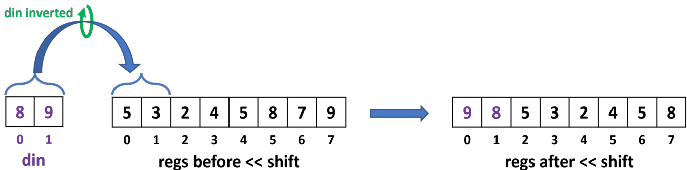
Illustration 43: Left-shifting Data Values
