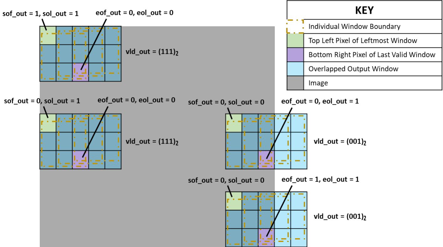
Illustration 52: Output Flags for Different Window Positions, without Boundary Padding
