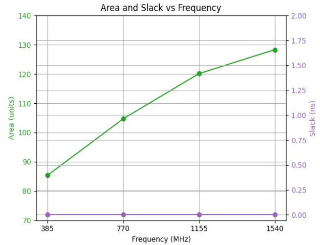
Illustration 49: Area and Slack vs Frequency
