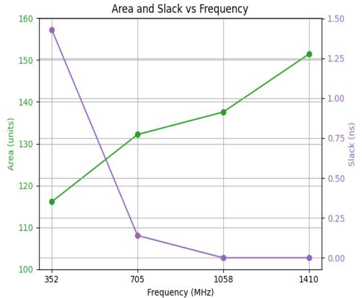
Illustration 39: Area and Slack vs Frequency
