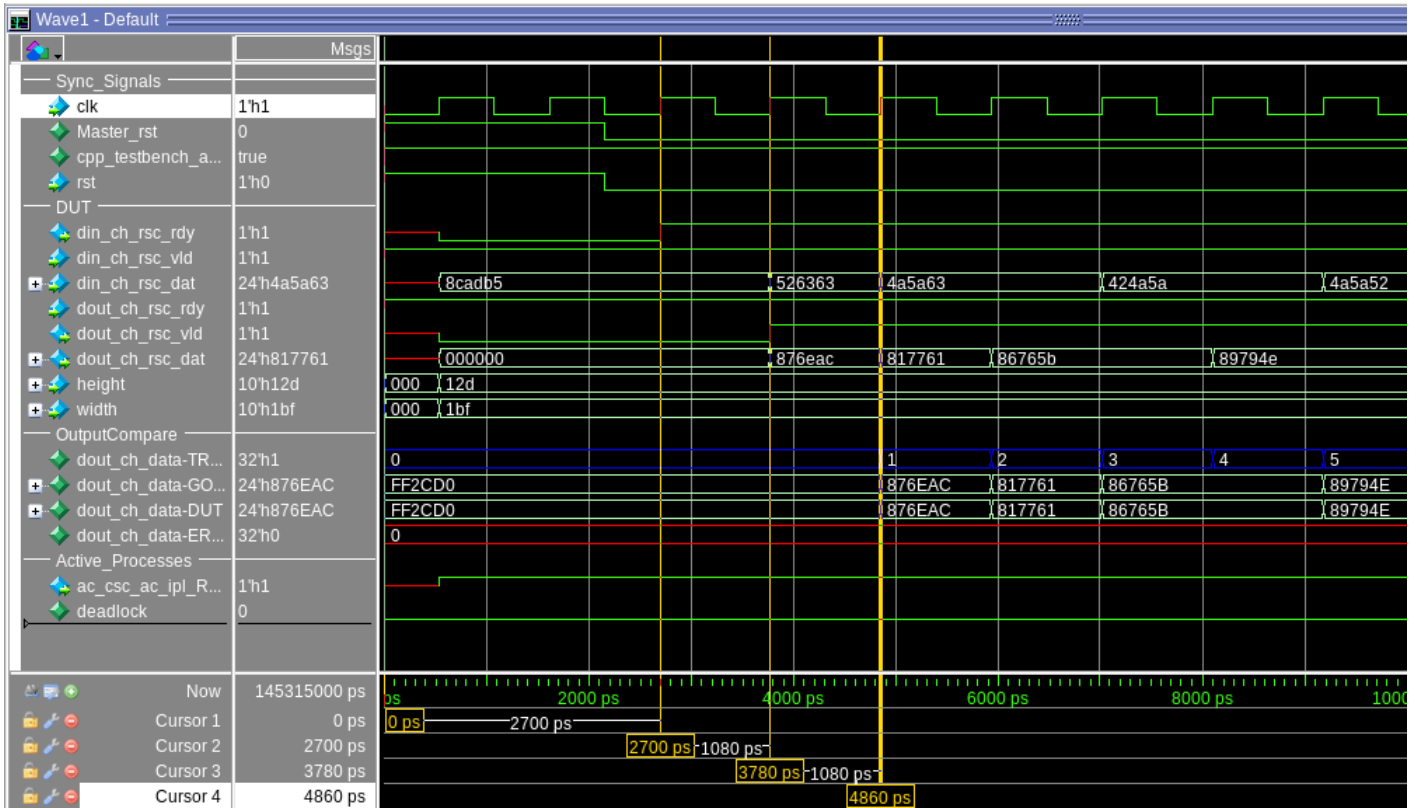
Illustration 7: RTL waveform
