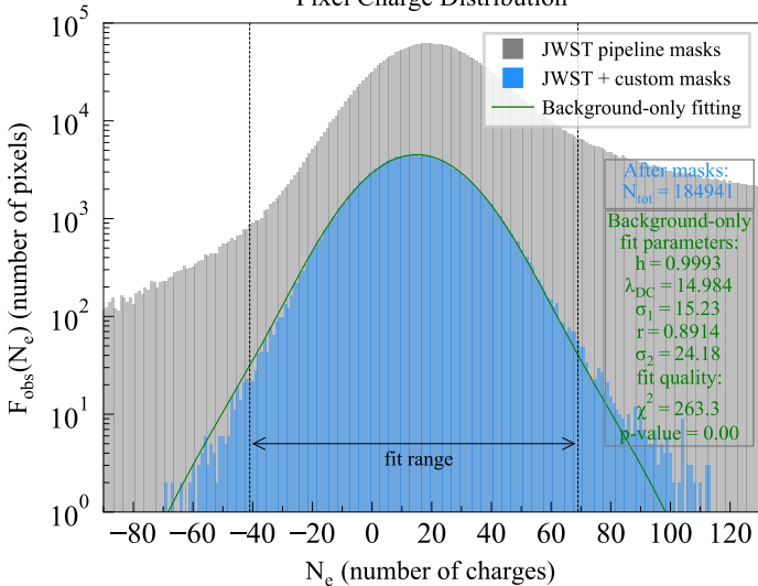
Pixel Charge Distribution
