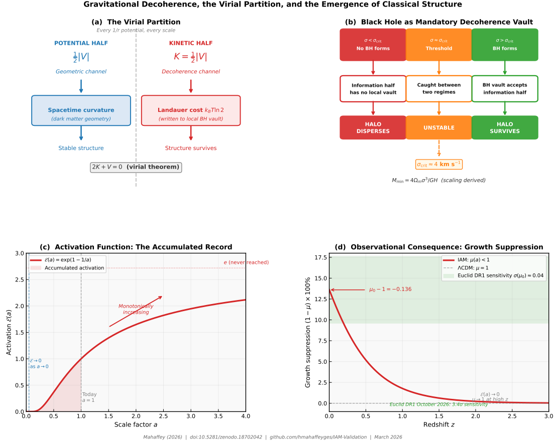
Figure 1: The virial partition and halo survival. Panel (a): the virial partition separates every bound 1/r system into a geometric channel (potential half, deposited into spacetime curvature) and an informational channel (kinetic half, the Landauer cost of the quantum-to-classical transition). Panel (b): the black hole as mandatory encoding vault — halos above \sigma_{\text{crit}} \approx 4 \text{ km s}^{-1} can form a local vault and survive; below this threshold the informational half has nowhere to write and the halo disperses. Panel (c): the activation function \mathcal{E}(a) = \exp(1 - 1/a) , the accumulated ledger of all decoherence transactions since the electroweak transition — the derived arrow of time. Panel (d): the observational consequence, growth suppression \mu(a) < 1 in the matter sector, falsifiable by Euclid DR1 (October 2026) at 3.4\sigma sensitivity.
