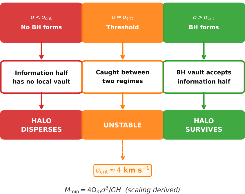
(b) Black Hole as Mandatory Decoherence Vault
