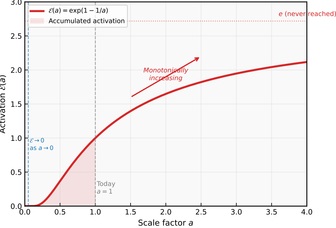
(c) Activation Function: The Accumulated Record
