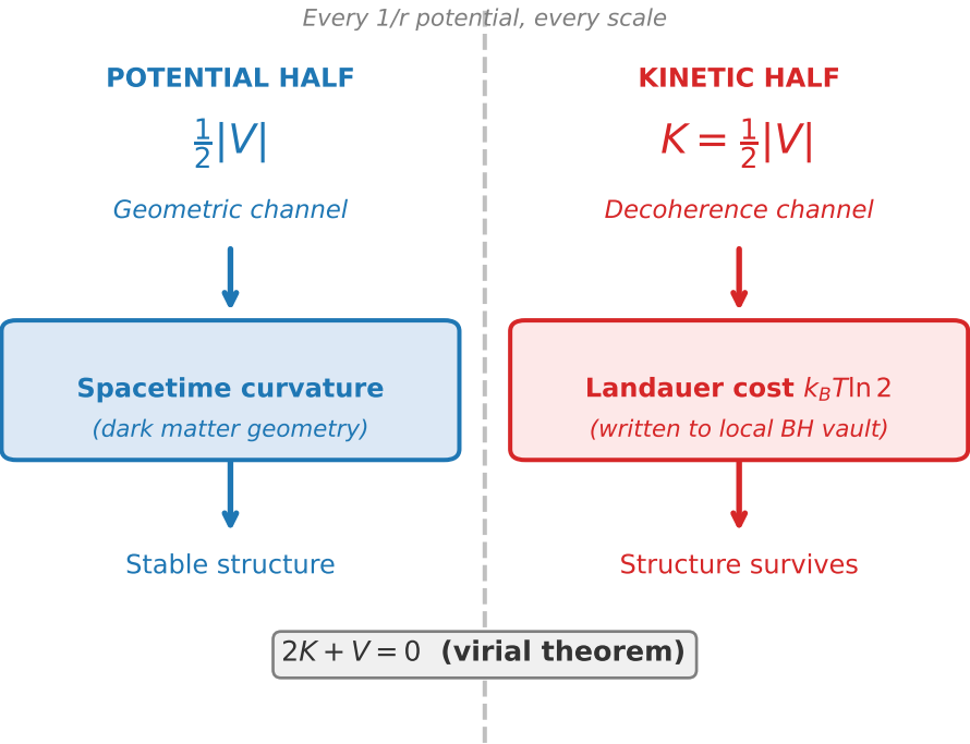
(a) The Virial Partition
