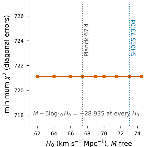
b The magnitudes do not choose H_0
