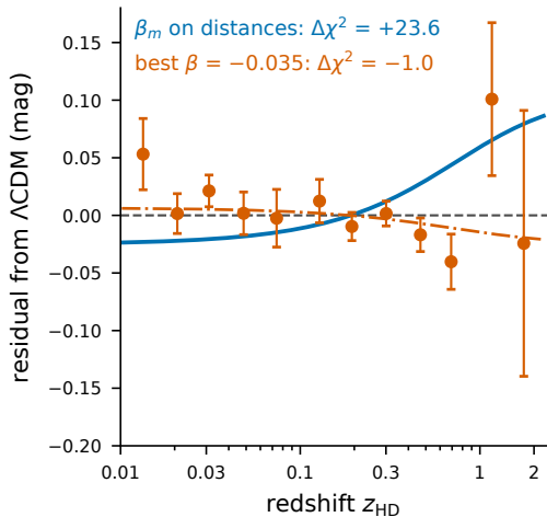
a Hubble-flow shape: \Lambda CDM geometry
