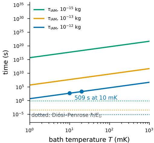
a \tau_{\text{IAM}} \propto T^2 ; Diósi-Penrose is flat
