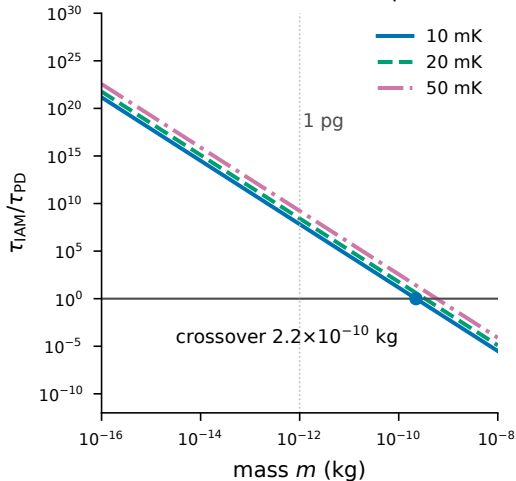
b Where the two channels separate
